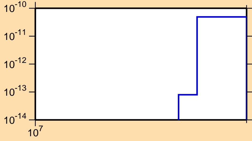
\sigma vs. E for ^{132}\text{Ba}(n,\text{pd})
