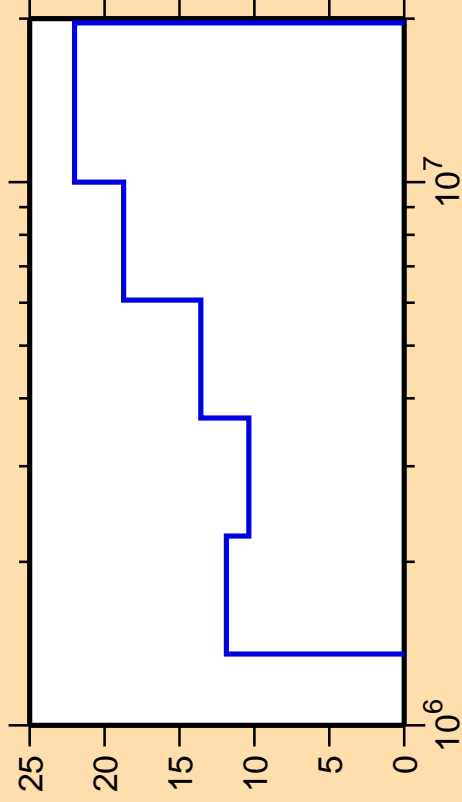
\Delta\sigma/\sigma vs. E for ^{132}\text{Ba}(n,n_4)
