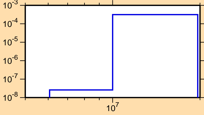
\sigma vs. E for ^{132}\text{Ba}(n,n\alpha)
