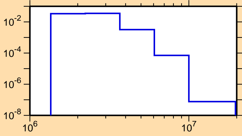
\sigma vs. E for ^{132}\text{Ba}(n,n_4)
