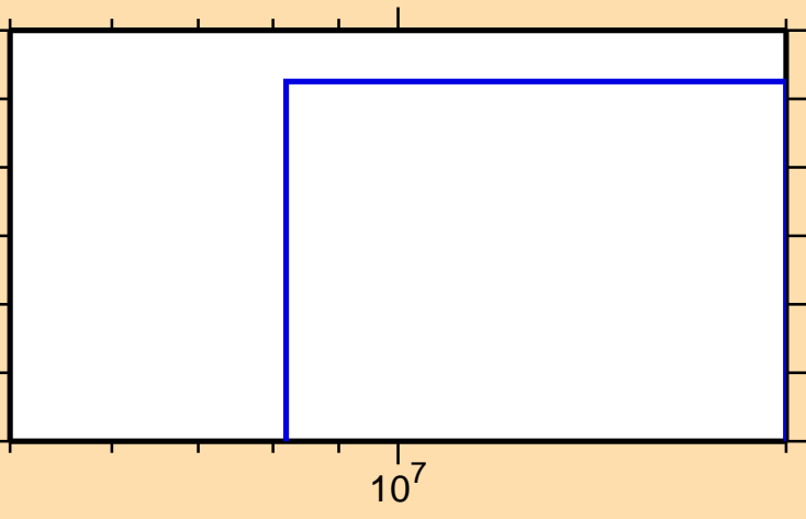
\sigma vs. E for ^{132}\text{Ba}(n,3n)
