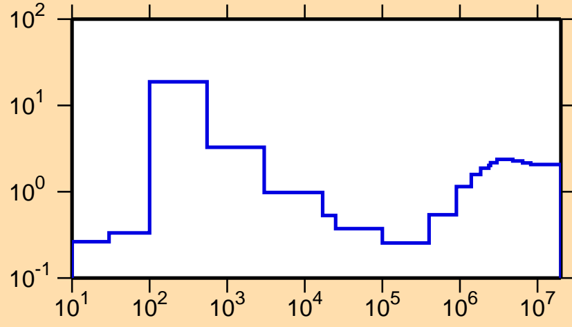
\sigma vs. E for ^{132}\text{Ba}(n,\text{nonel.})
