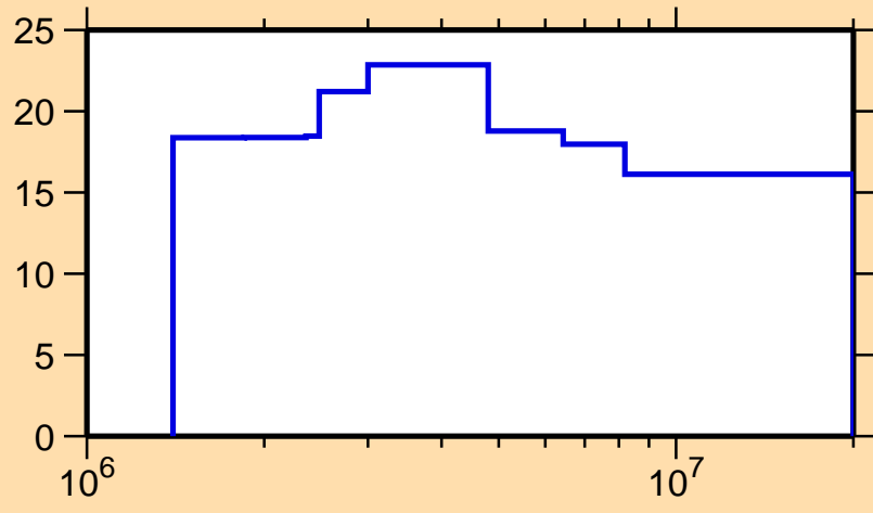
\Delta\sigma/\sigma vs. E for ^{132}\text{Ba}(n,n_1)
