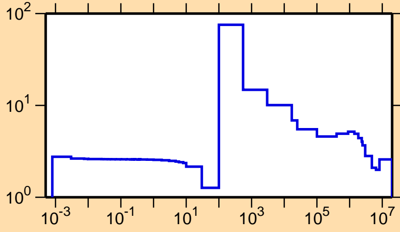
\sigma vs. E for ^{132}\text{Ba}(n,\text{el.})
