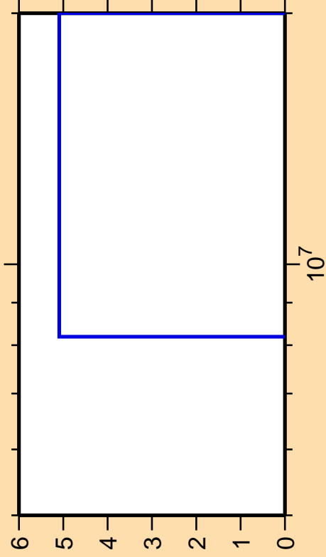
\Delta\sigma/\sigma vs. E for ^{132}\text{Ba}(n,2n)
