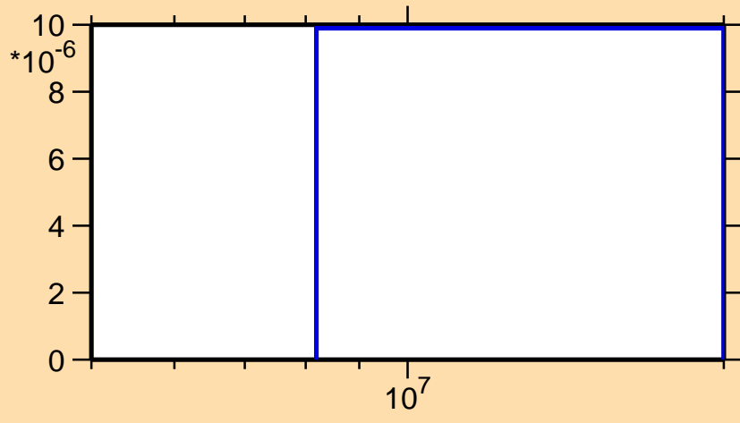
\sigma vs. E for ^{132}\text{Ba}(n,t)
