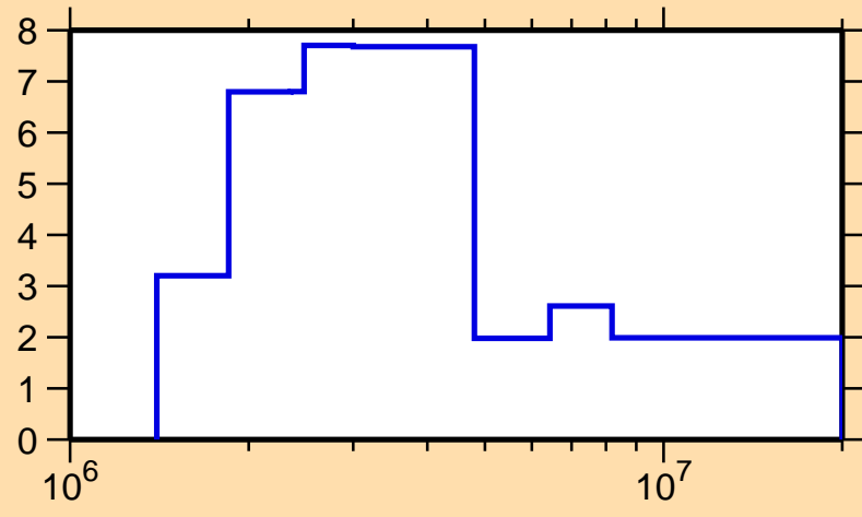
\Delta\sigma/\sigma vs. E for ^{132}\text{Ba}(n,\text{el.})
