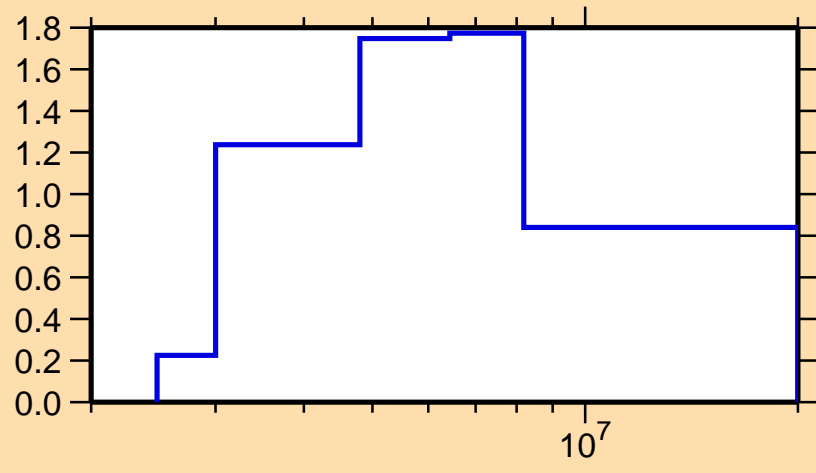
\sigma vs. E for ^{132}\text{Ba}(n,n\text{cont.})
