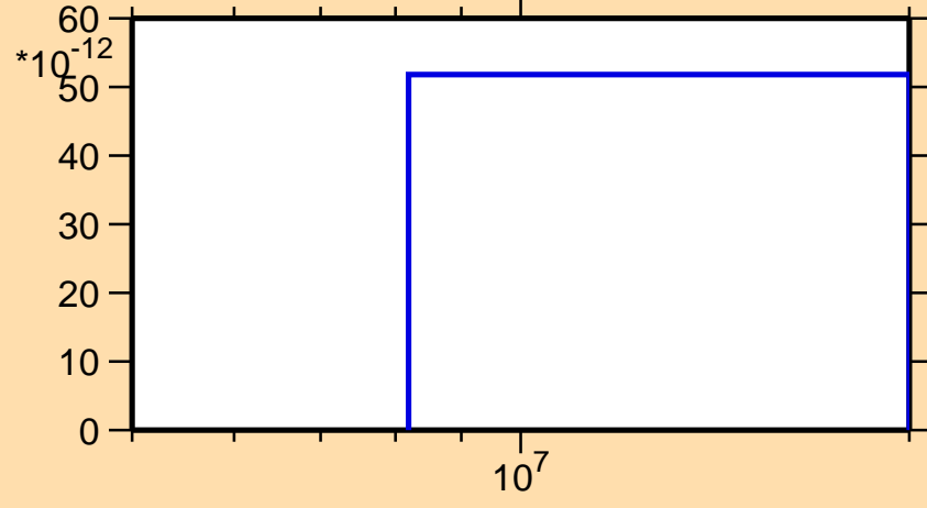
\sigma vs. E for ^{132}\text{Ba}(n,p\alpha)
