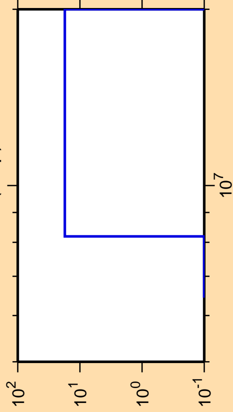
\Delta\sigma/\sigma vs. E for ^{132}\text{Ba}(n,np)
