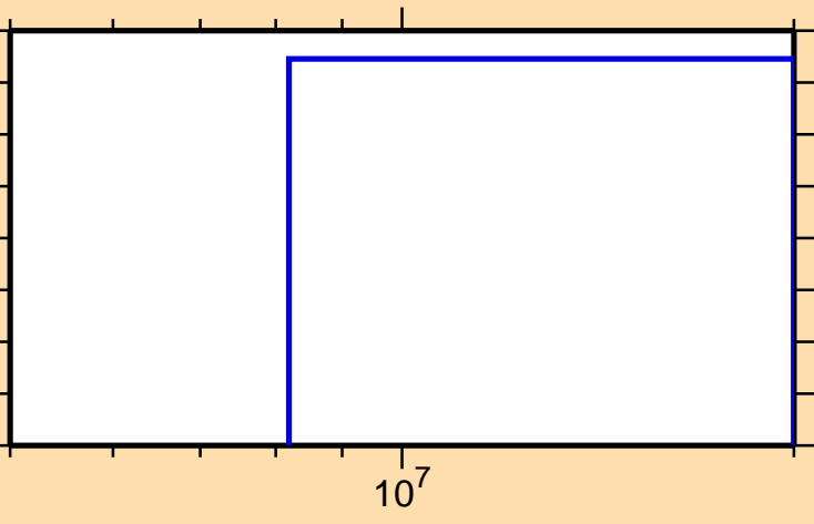
\sigma vs. E for ^{132}\text{Ba}(n,2np)
