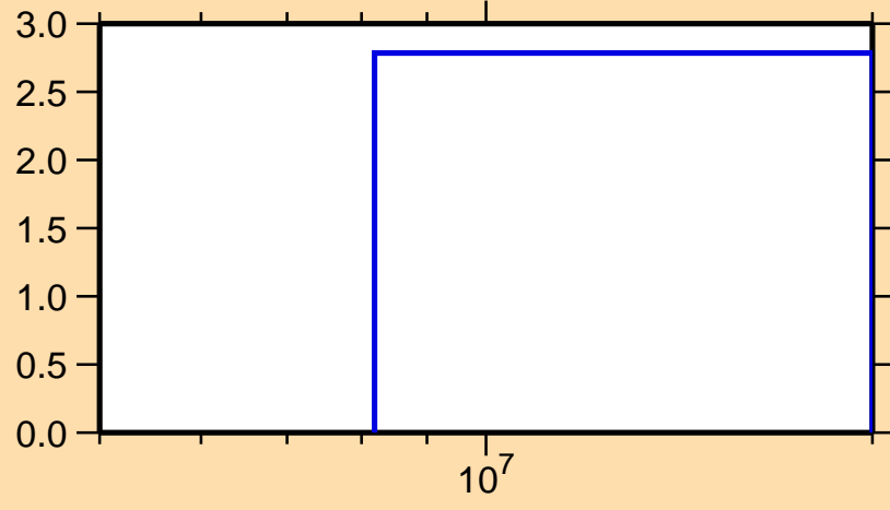
\Delta\sigma/\sigma vs. E for ^{132}\text{Ba}(n,\text{nonel.})
