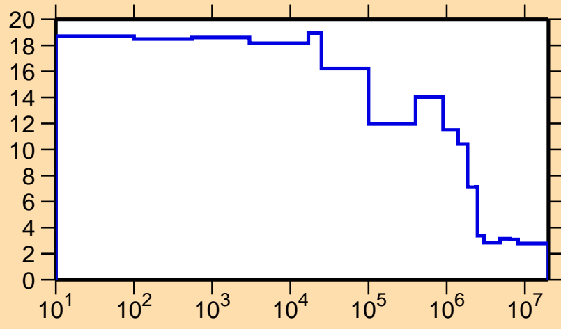
\Delta\sigma/\sigma vs. E for ^{132}\text{Ba}(n,\text{nonel.})
