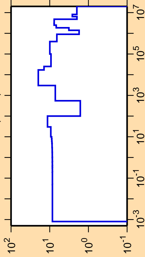
\Delta\sigma/\sigma vs. E for ^{132}\text{Ba}(n,\text{el.})
