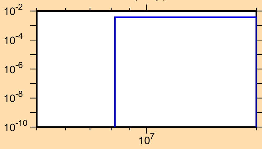
\sigma vs. E for ^{132}\text{Ba}(n,np)
