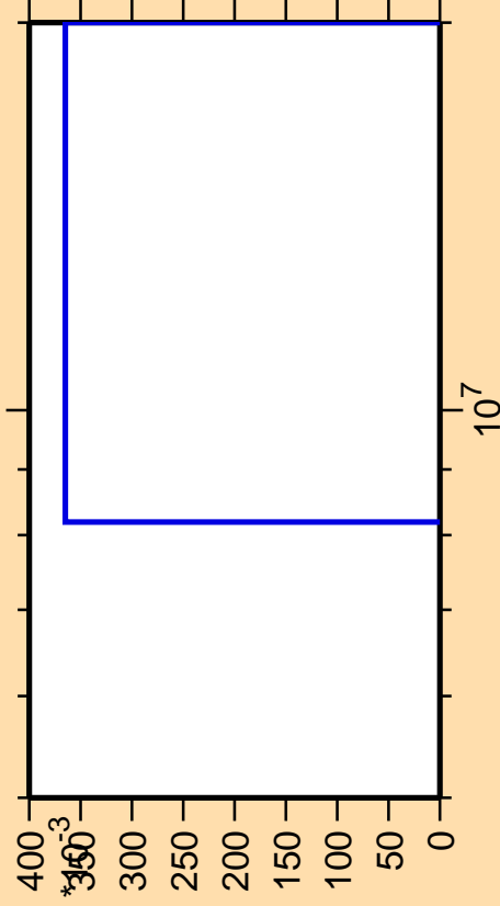
\Delta\sigma/\sigma vs. E for ^{132}\text{Ba}(n,pd)
