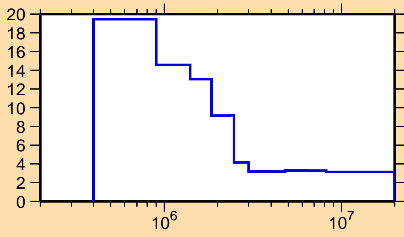
\Delta\sigma/\sigma vs. E for ^{132}\text{Ba}(n,\text{inel.})
