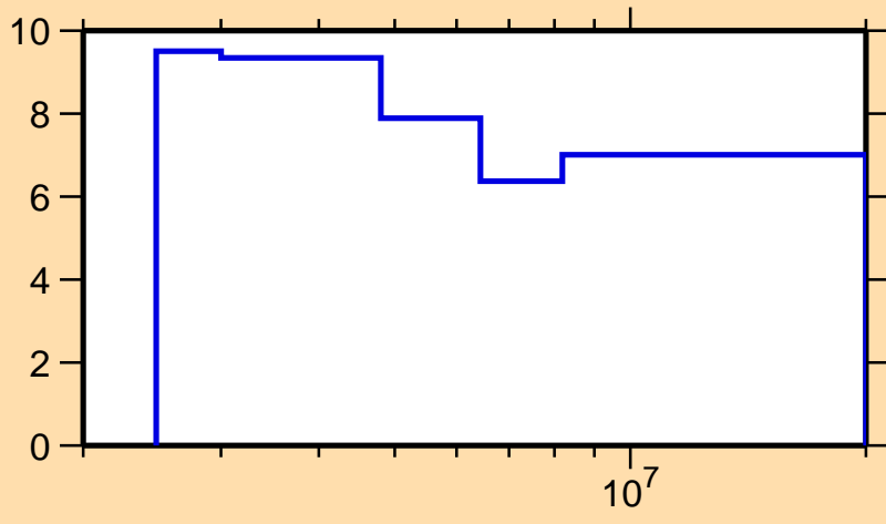
\Delta\sigma/\sigma vs. E for ^{132}\text{Ba}(n,n\text{cont.})
