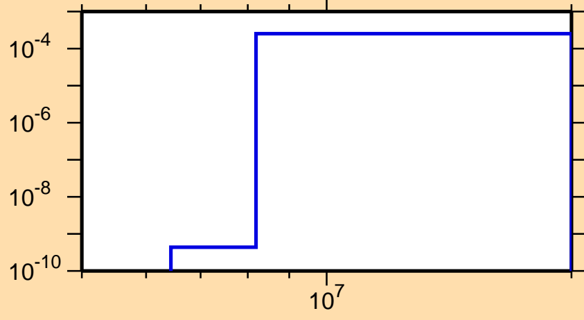
\sigma vs. E for ^{132}\text{Ba}(n,n\alpha)
