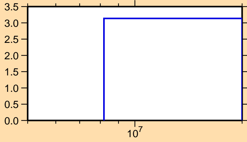
\Delta\sigma/\sigma vs. E for ^{132}\text{Ba}(n,\text{inel.})
