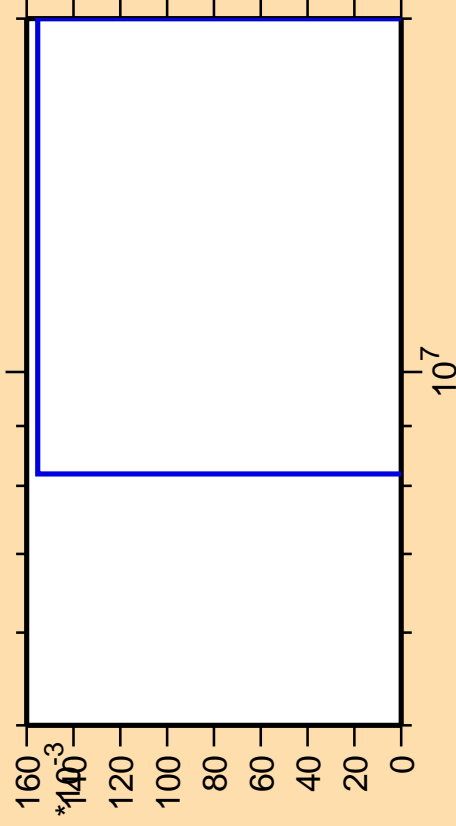
\Delta\sigma/\sigma vs. E for ^{132}\text{Ba}(n,nt)
