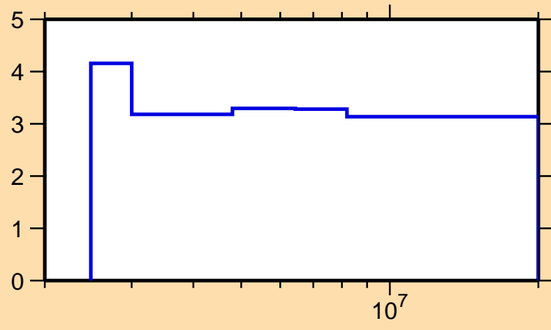
\Delta\sigma/\sigma vs. E for ^{132}\text{Ba}(n,\text{inel.})
