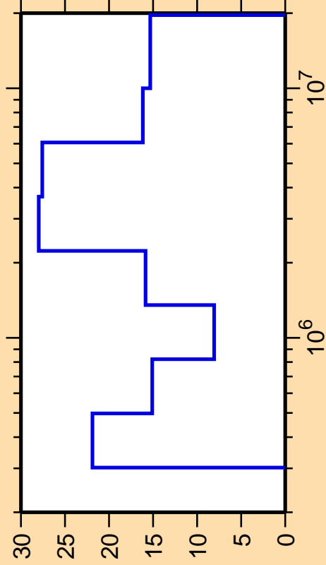
\Delta\sigma/\sigma vs. E for ^{133}\text{Ba}(n,n_2)
