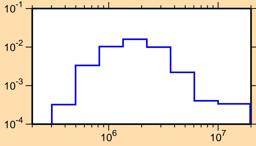
\sigma vs. E for ^{133}\text{Ba}(n,n_2)
