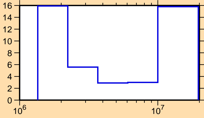
\Delta\sigma/\sigma vs. E for ^{135}\text{Ba}(n,n\text{cont.})
