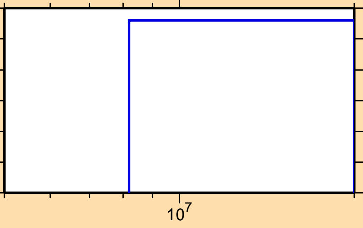
\sigma vs. E for ^{135}\text{Ba}(n,t)
