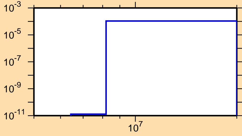
\sigma vs. E for ^{135}\text{Ba}(n,n\alpha)
