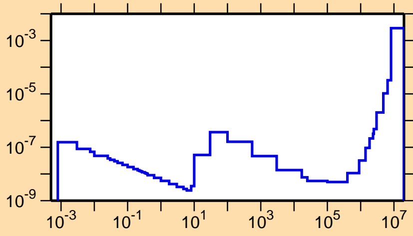
\sigma vs. E for ^{135}\text{Ba}(n,\alpha)
