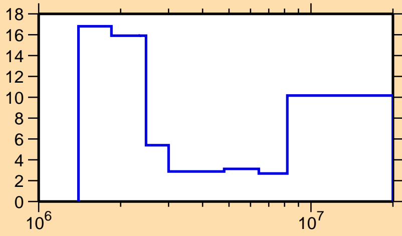
\Delta\sigma/\sigma vs. E for ^{135}\text{Ba}(n,n\text{cont.})
