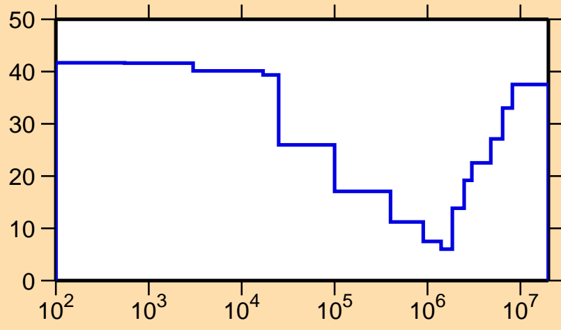
\Delta\sigma/\sigma vs. E for ^{135}\text{Ba}(n,n_1)
