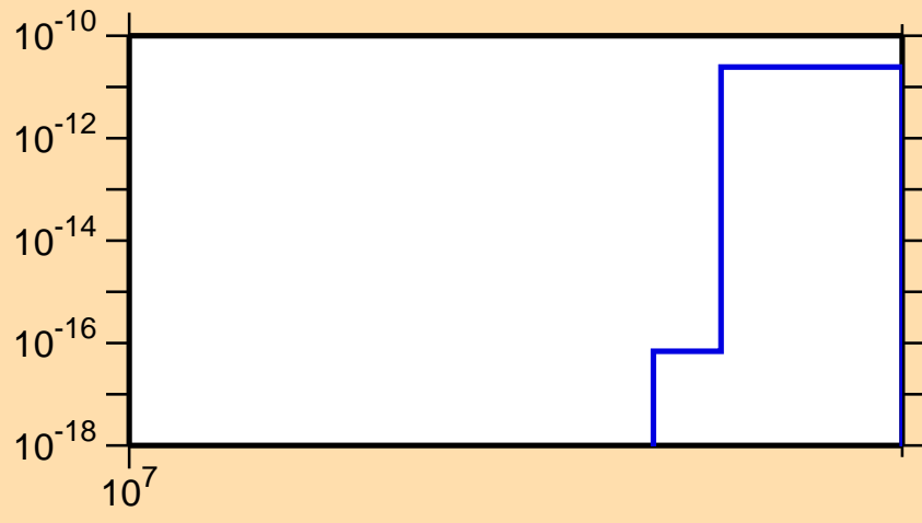
\sigma vs. E for ^{136}\text{Ba}(n,nt)
