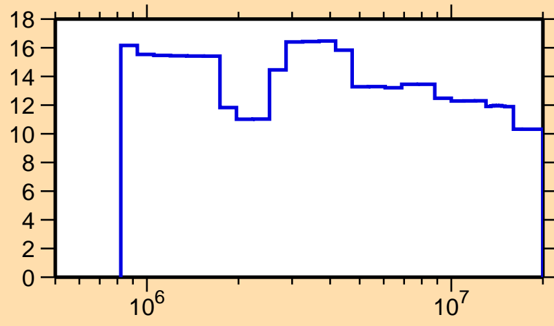
\Delta\sigma/\sigma vs. E for ^{136}\text{Ba}(n,n_1)
