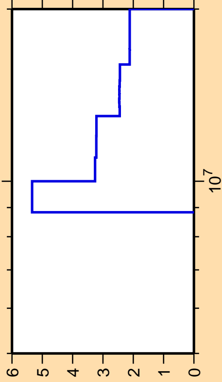
\Delta\sigma/\sigma vs. E for ^{136}\text{Ba}(n,2n)
