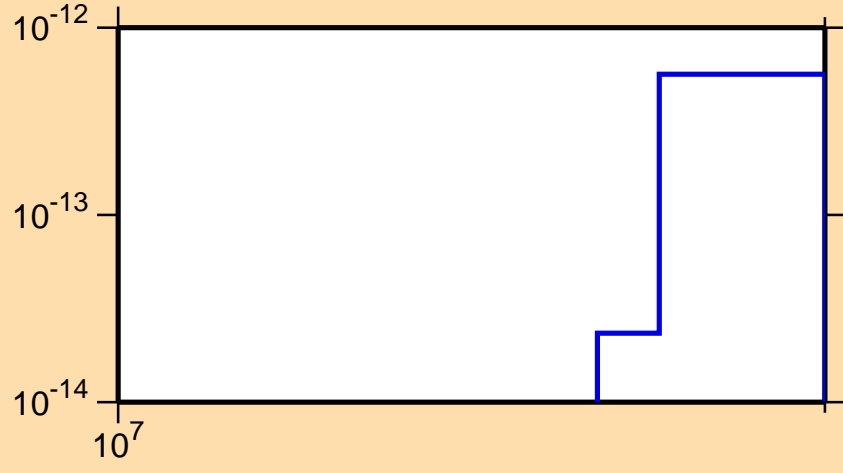
\sigma vs. E for ^{136}\text{Ba}(n,p\alpha)
