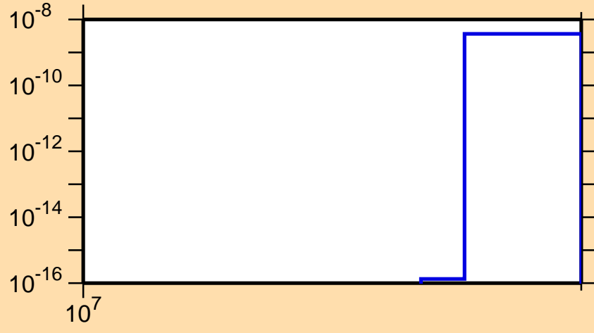
\sigma vs. E for ^{136}\text{Ba}(n,\text{nd})
