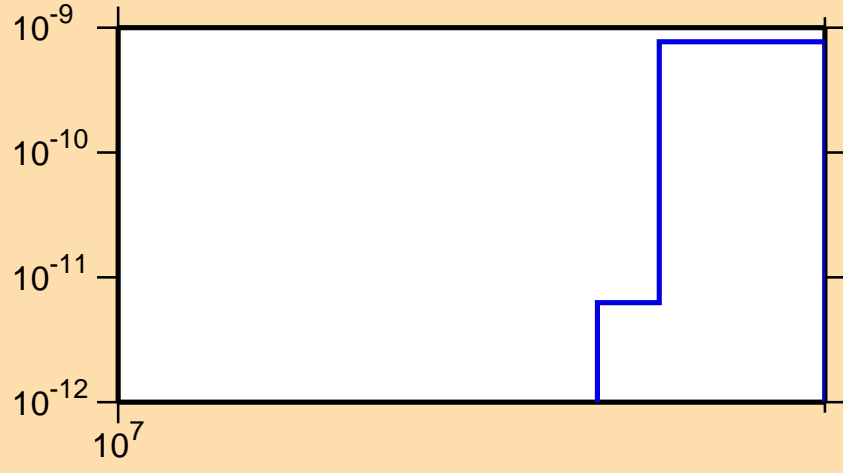
\sigma vs. E for ^{136}\text{Ba}(n,\text{He3})
