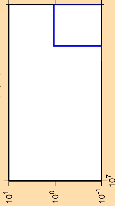
\Delta\sigma/\sigma vs. E for ^{136}\text{Ba}(n,p\alpha)
