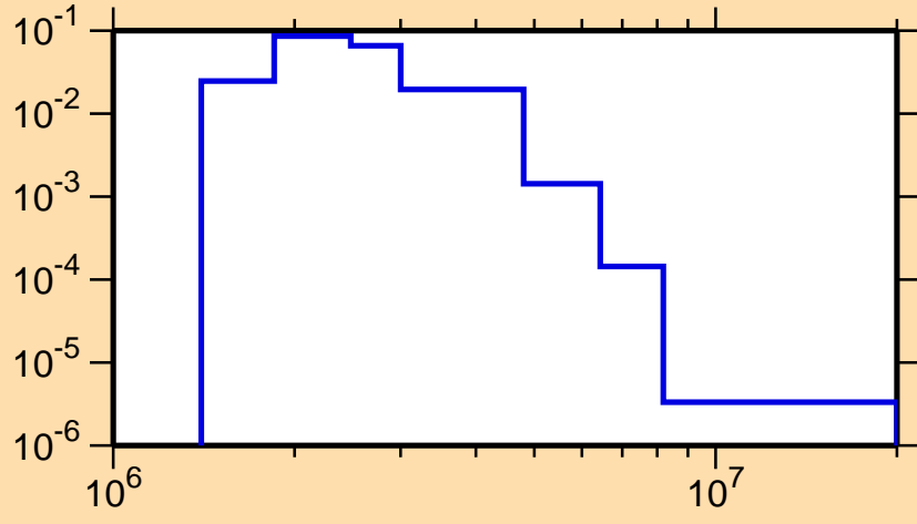
\sigma vs. E for ^{136}\text{Ba}(n,n_3)
