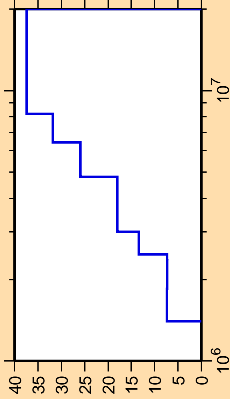
\Delta\sigma/\sigma vs. E for ^{136}\text{Ba}(n,n_3)
