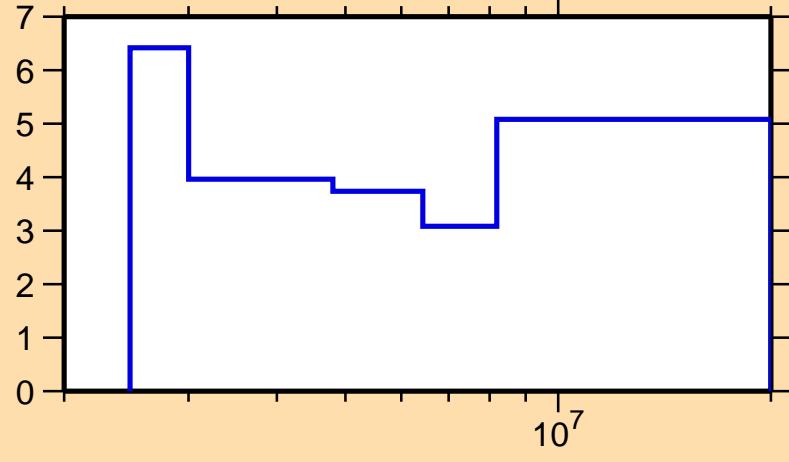
\Delta\sigma/\sigma vs. E for ^{136}\text{Ba}(n,n\text{cont.})
