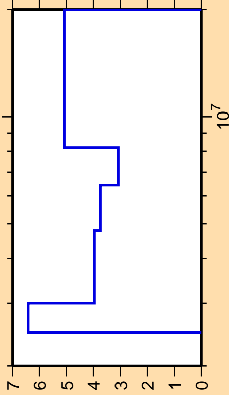
\Delta\sigma/\sigma vs. E for ^{136}\text{Ba}(n,n\text{cont.})
