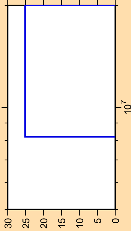
\Delta\sigma/\sigma vs. E for ^{136}\text{Ba}(n,nd)
