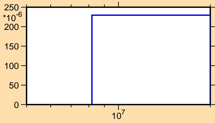
\sigma vs. E for ^{136}\text{Ba}(n,np)
