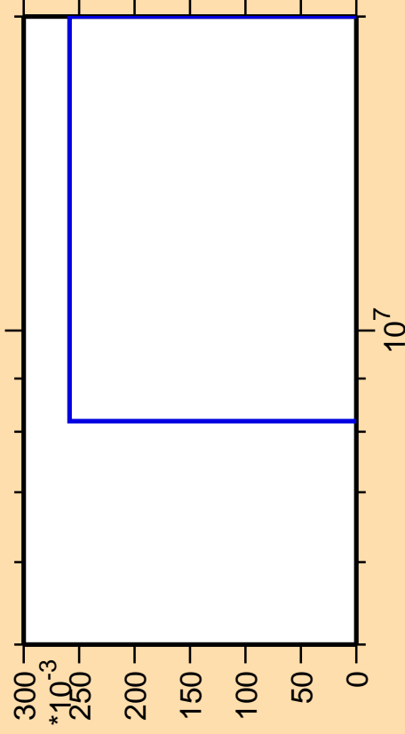
\Delta\sigma/\sigma vs. E for ^{136}\text{Ba}(n,nt)
