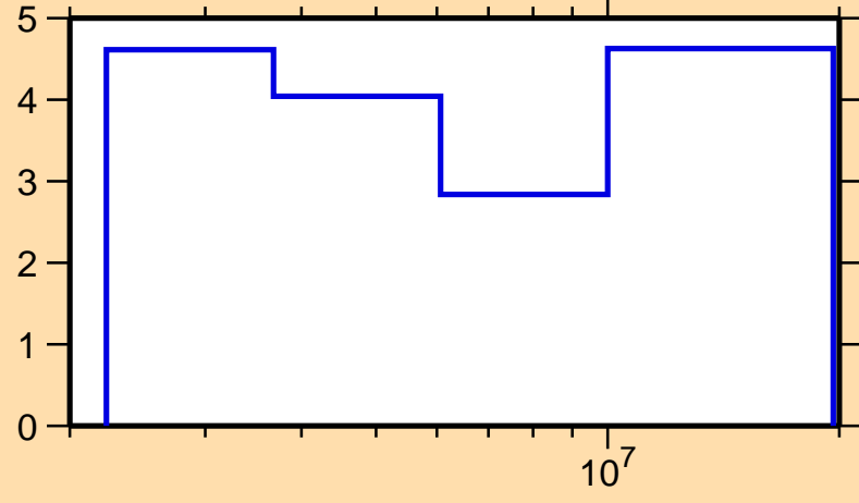
\Delta\sigma/\sigma vs. E for ^{137}\text{Ba}(n,n\text{cont.})
