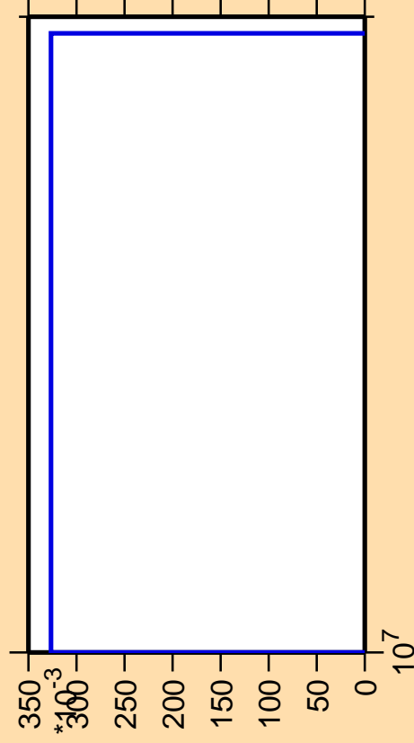
\Delta\sigma/\sigma vs. E for ^{137}\text{Ba}(n,nt)
