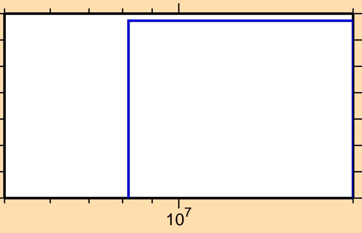
\sigma vs. E for ^{137}\text{Ba}(n,np)
