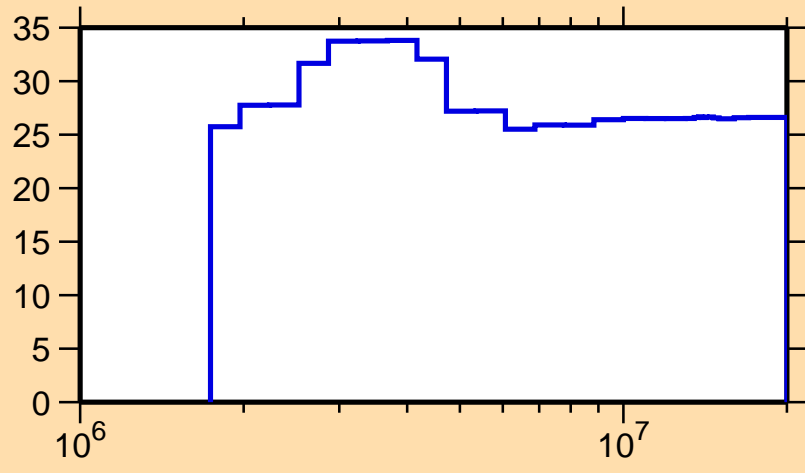
\Delta\sigma/\sigma vs. E for ^{138}\text{Ba}(n,\gamma)
