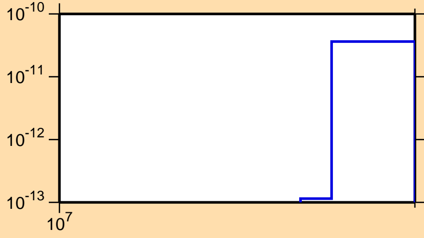
\sigma vs. E for ^{138}\text{Ba}(n,\text{He3})
