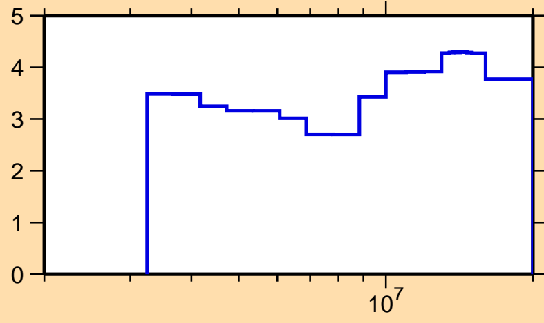
\Delta\sigma/\sigma vs. E for ^{138}\text{Ba}(n,\text{inel.})
