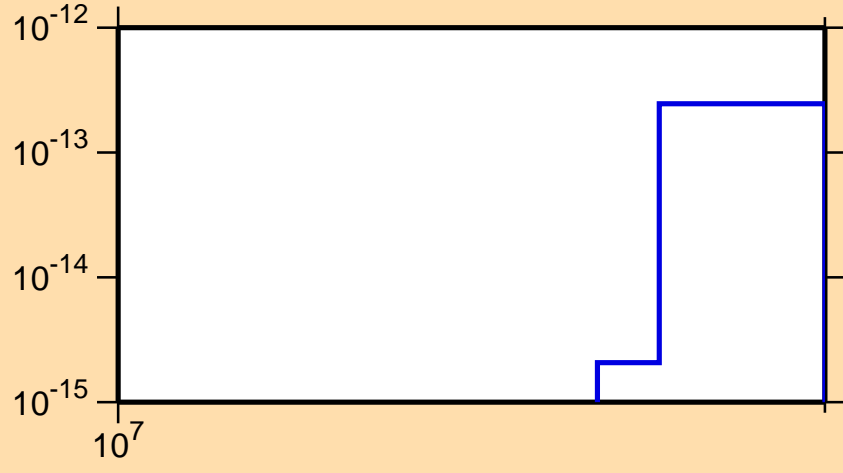
\sigma vs. E for ^{138}\text{Ba}(n,p\alpha)
