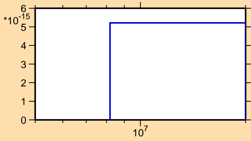
\sigma vs. E for ^{138}\text{Ba}(n,2np)
