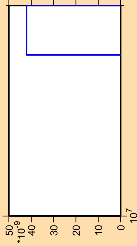
\Delta\sigma/\sigma vs. E for ^{139}\text{Ba} (mt 11)
