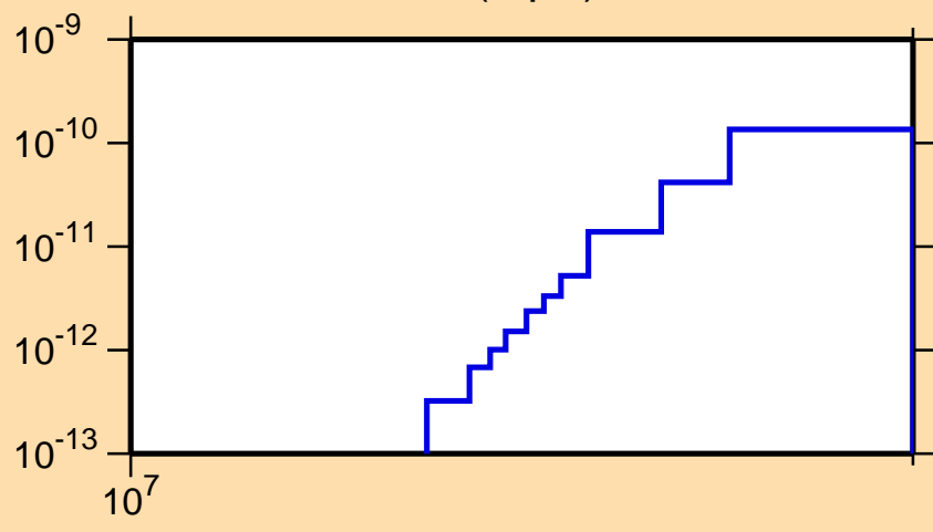
\sigma vs. E for ^{139}\text{Ba}(n,p\alpha)
