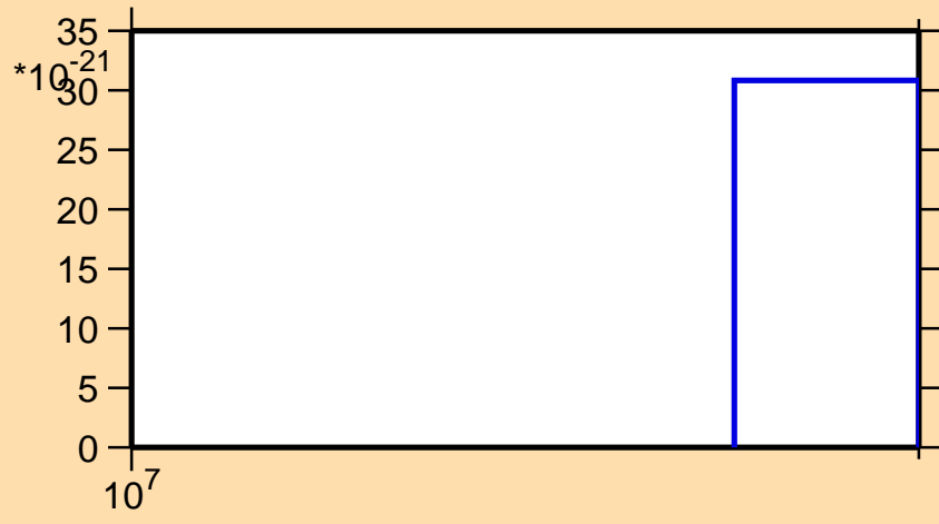
\sigma vs. E for ^{139}\text{Ba} (mt 11)
