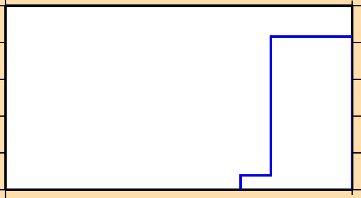
\sigma vs. E for ^{139}\text{Ba}(n,nt)
