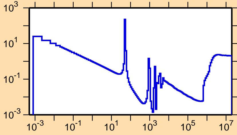
\sigma vs. E for ^{139}\text{Ba}(n,\text{nonel.})
