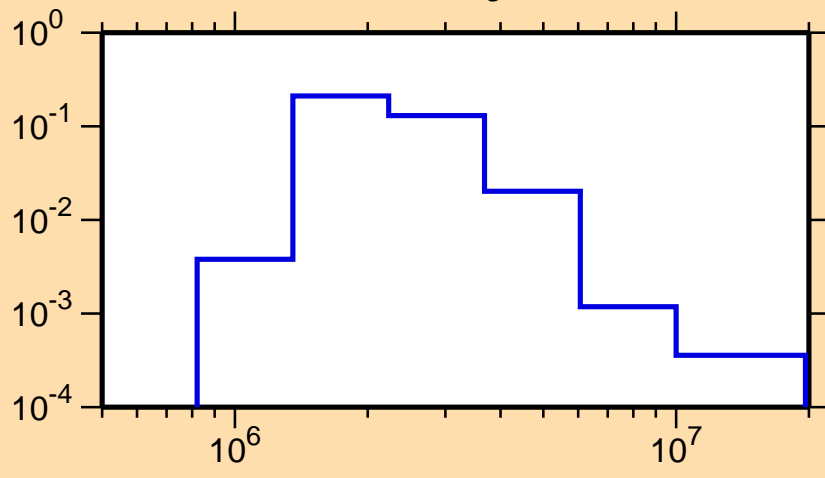
\sigma vs. E for ^{139}\text{Ba}(n,n_3)
