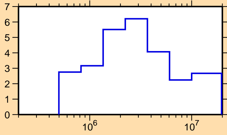
\Delta\sigma/\sigma vs. E for ^{139}\text{Ba}(n,\text{el.})
