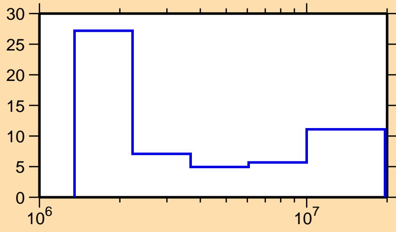
\Delta\sigma/\sigma vs. E for ^{139}\text{Ba}(n,n\text{cont.})
