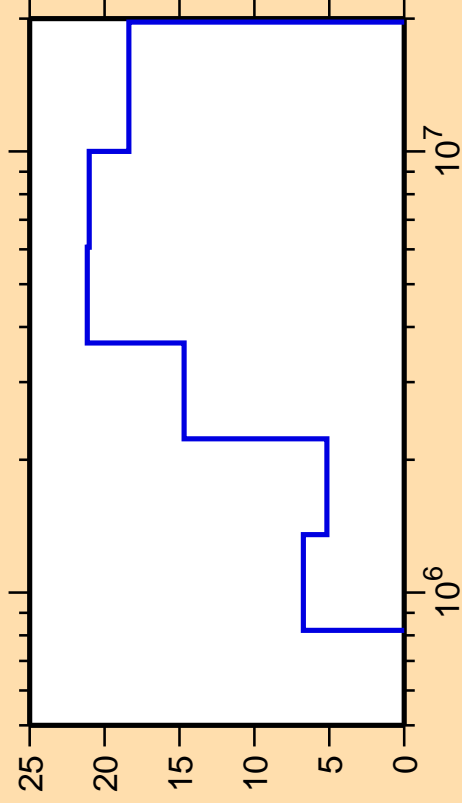
\Delta\sigma/\sigma vs. E for ^{139}\text{Ba}(n,n_4)
