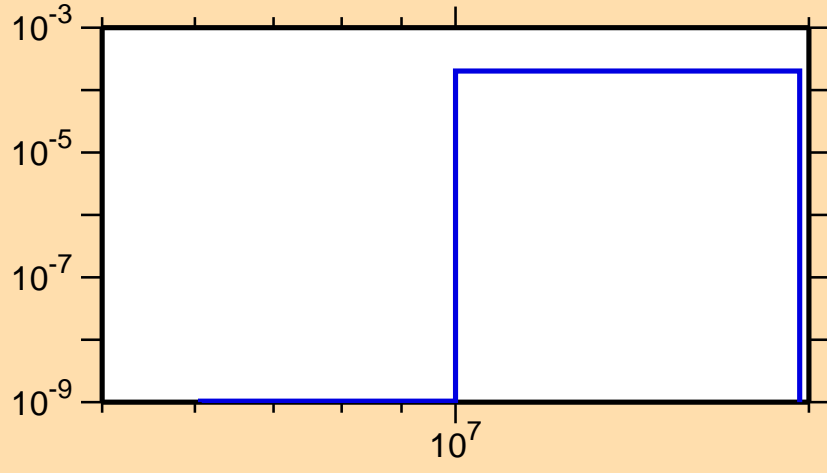
\sigma vs. E for ^{139}\text{Ba}(n,n\alpha)
