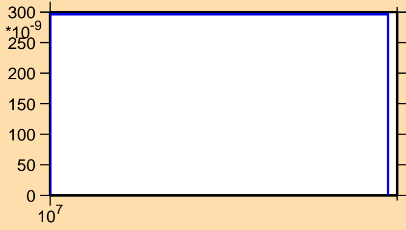
\sigma vs. E for ^{139}\text{Ba}(n,\text{nd})
