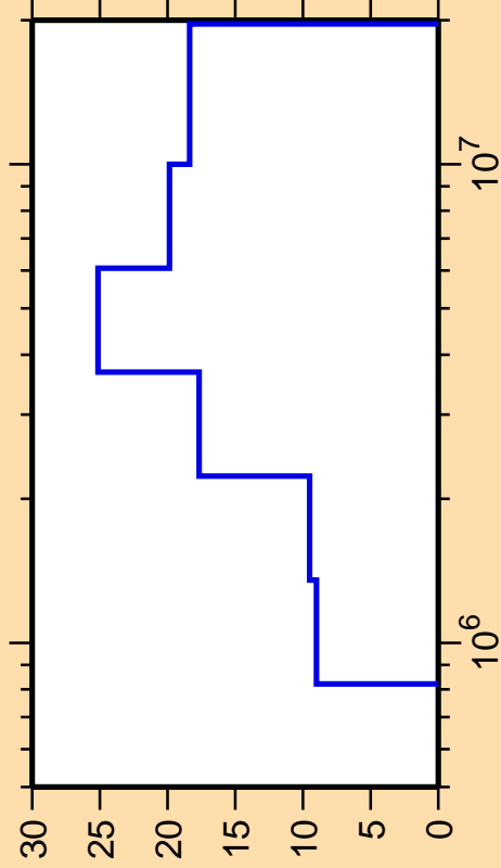
\Delta\sigma/\sigma vs. E for ^{139}\text{Ba}(n,n_3)
