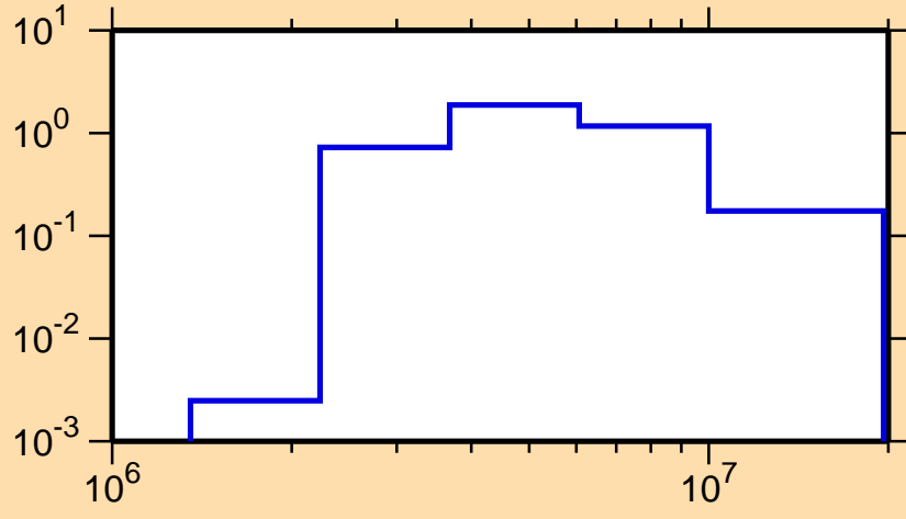
\sigma vs. E for ^{139}\text{Ba}(n,n\text{cont.})
