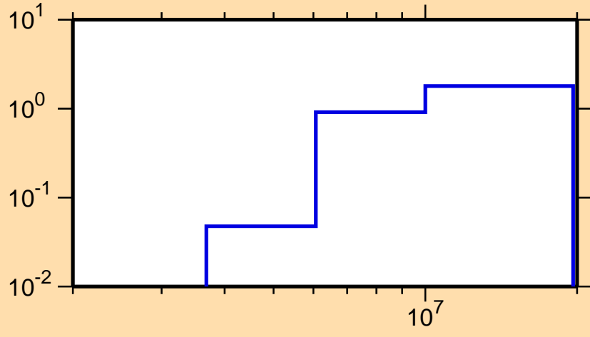
\sigma vs. E for ^{139}\text{Ba}(n,2n)
