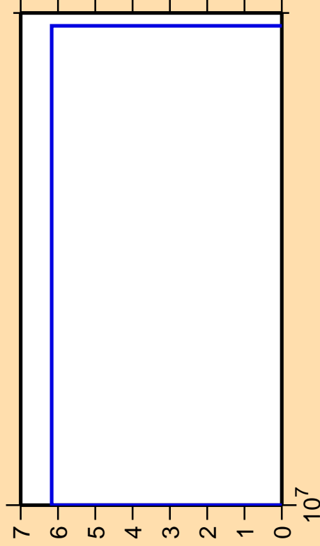
\Delta\sigma/\sigma vs. E for ^{139}\text{Ba}(n,3n)
