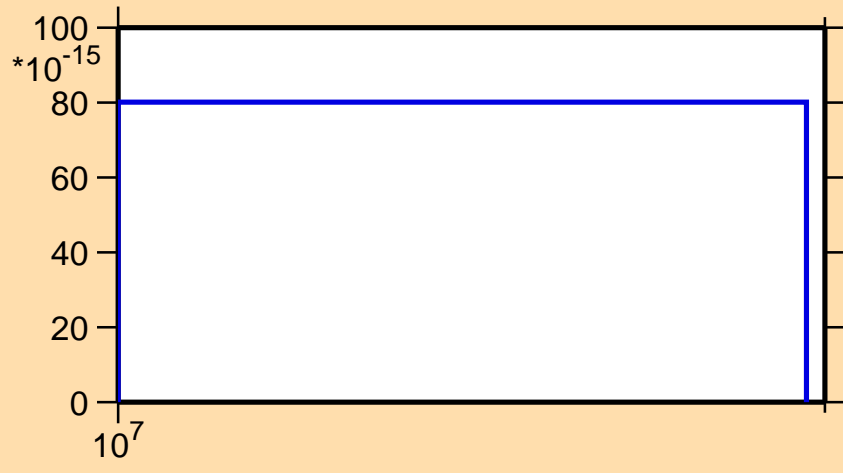
\sigma vs. E for ^{139}\text{Ba}(n,\text{He}3)
