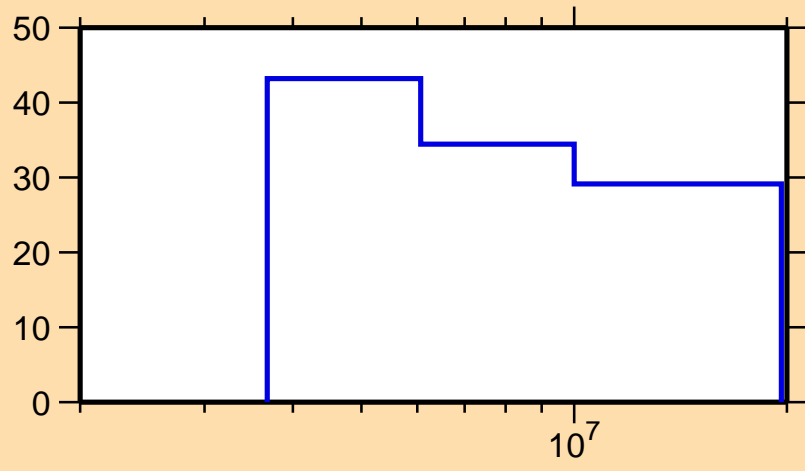
\Delta\sigma/\sigma vs. E for ^{139}\text{Ba}(n,p)
