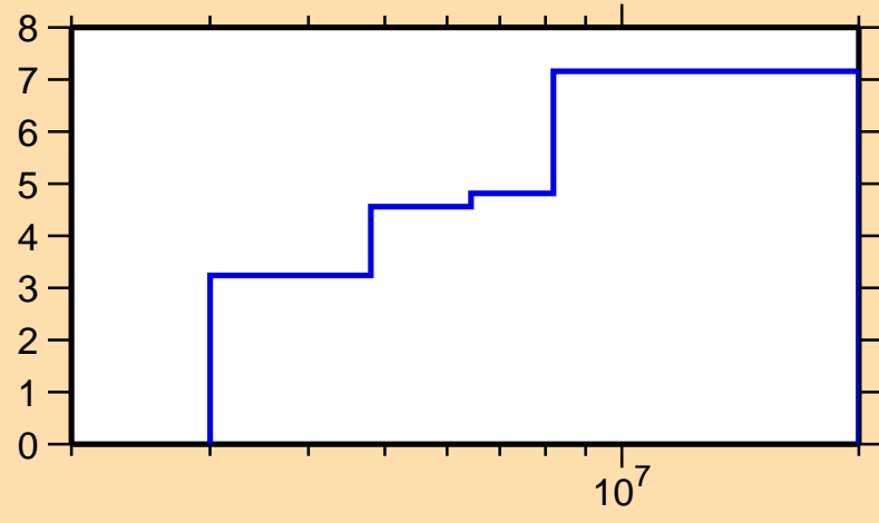
\Delta\sigma/\sigma vs. E for ^{139}\text{Ba}(n,\text{inel.})
