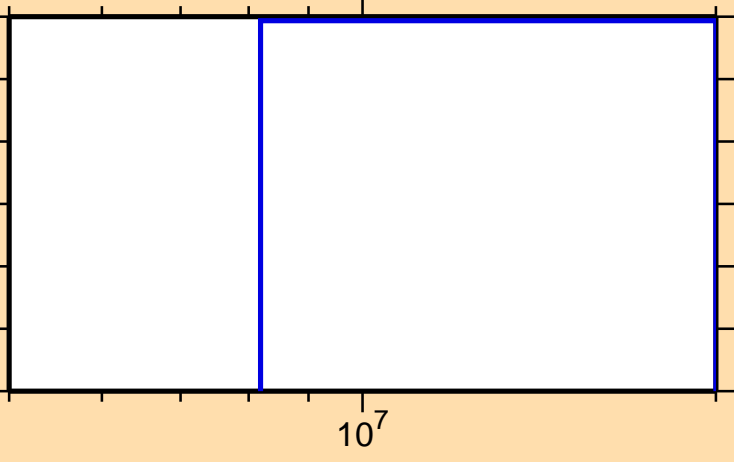
\sigma vs. E for ^{139}\text{Ba}(n,nt)
