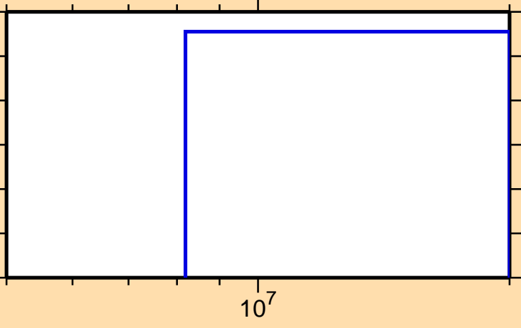
\sigma vs. E for ^{139}\text{Ba}(n,2n\alpha)
