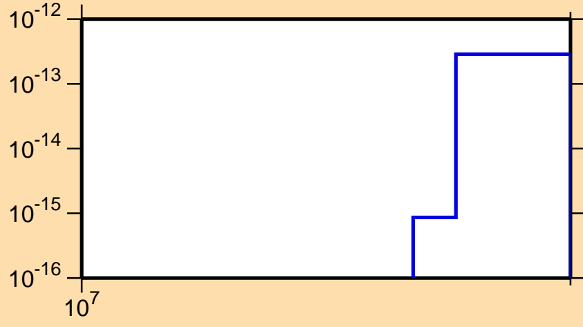
\sigma vs. E for ^{140}\text{Ba}(n,\text{He}3)
