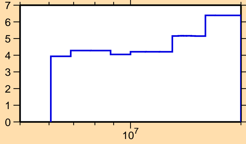
\Delta\sigma/\sigma vs. E for ^{140}\text{Ba}(n,\text{el.})
