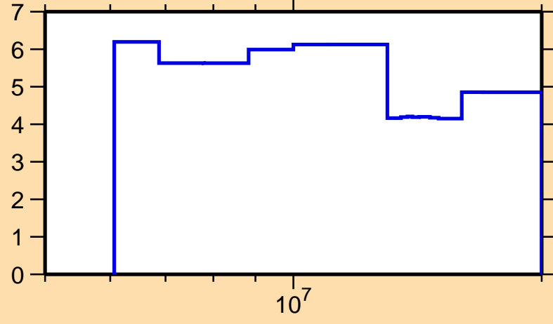
\Delta\sigma/\sigma vs. E for ^{140}\text{Ba}(n,\text{nonel.})
