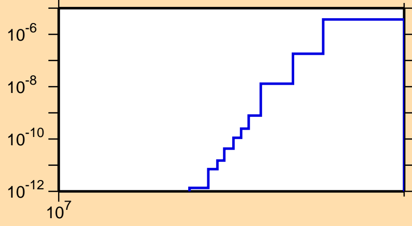
\sigma vs. E for ^{140}\text{Ba}(n,2n\alpha)
