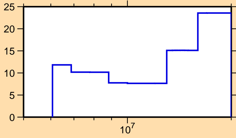
\Delta\sigma/\sigma vs. E for ^{140}\text{Ba}(n,2n)
