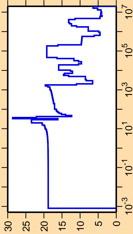
\Delta\sigma/\sigma vs. E for ^{140}\text{Ba}(n,\text{el.})
