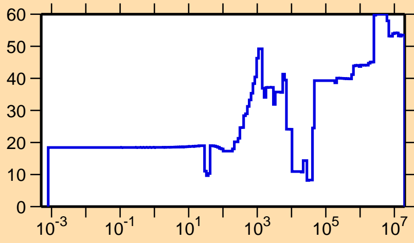
\Delta\sigma/\sigma vs. E for ^{140}\text{Ba}(n,\gamma)
