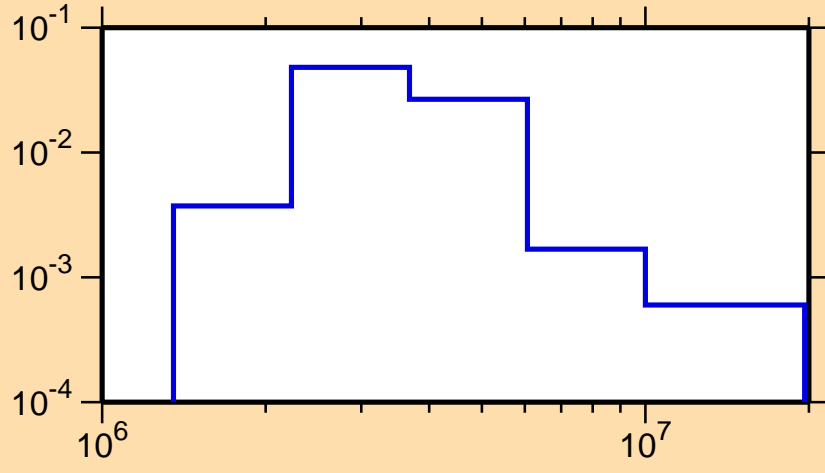
\sigma vs. E for ^{140}\text{Ba}(n,n_4)
