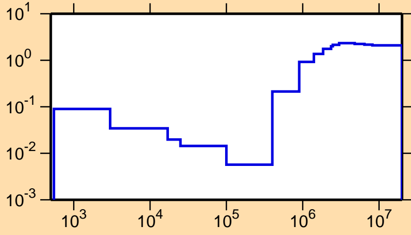
\sigma vs. E for ^{140}\text{Ba}(n,\text{nonel.})
