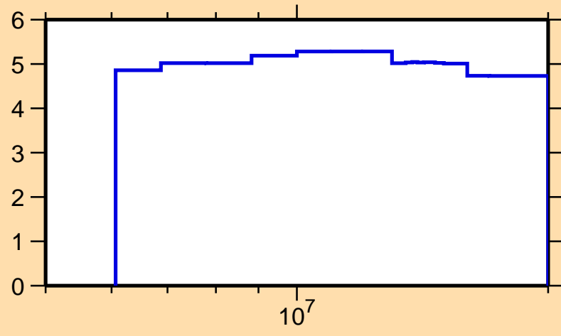
\Delta\sigma/\sigma vs. E for ^{141}\text{Ba}(n,\text{nonel.})
