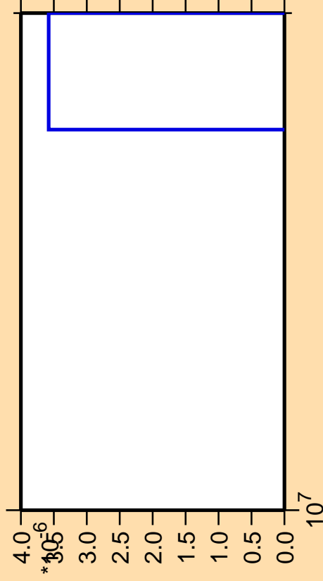
\Delta\sigma/\sigma vs. E for ^{141}\text{Ba} (mt 11)
