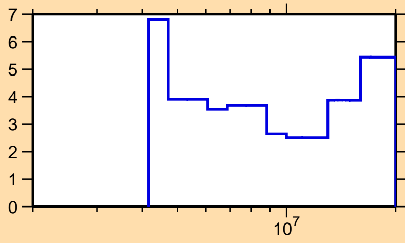
\Delta\sigma/\sigma vs. E for ^{141}\text{Ba}(n,\text{tot.})
