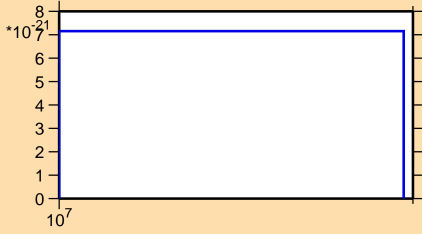
\sigma vs. E for ^{141}\text{Ba} (mt 11)
