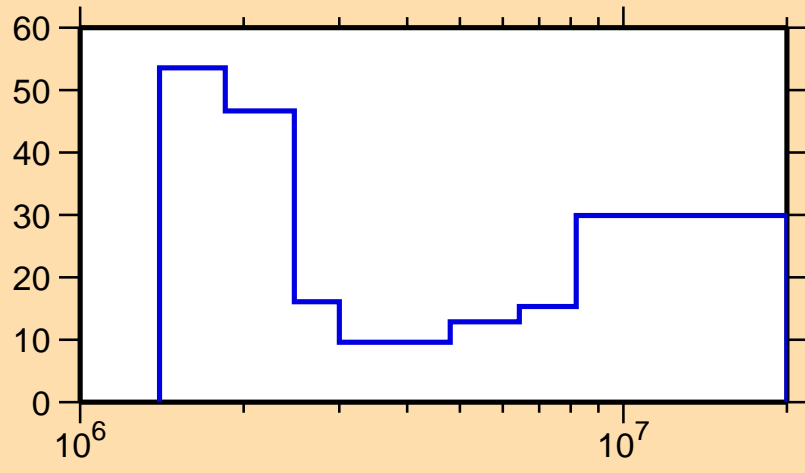
\Delta\sigma/\sigma vs. E for ^{141}\text{Ba}(n,n\text{cont.})
