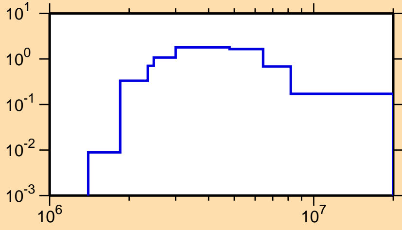
\sigma vs. E for ^{141}\text{Ba}(n,n\text{cont.})
