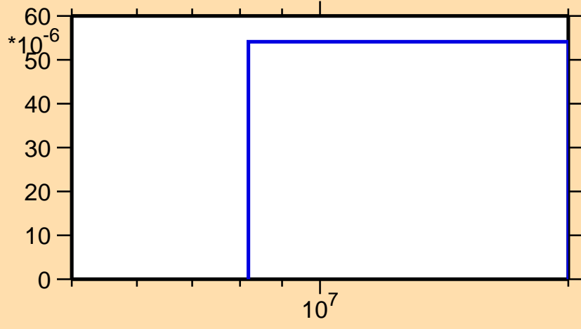
\sigma vs. E for ^{141}\text{Ba}(n,t)
