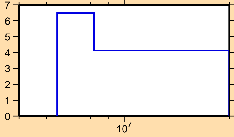
\Delta\sigma/\sigma vs. E for ^{141}\text{Ba}(n,\text{el.})
