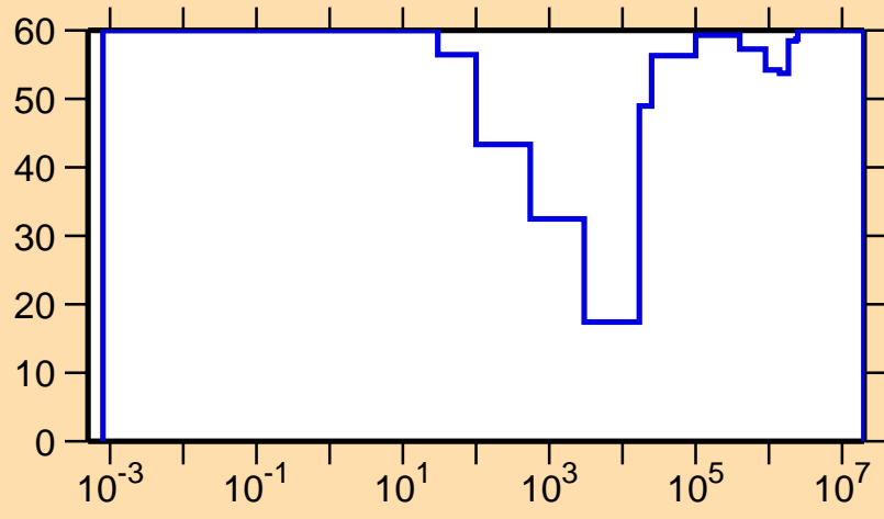
\Delta\sigma/\sigma vs. E for ^{141}\text{Ba}(n,\gamma)
