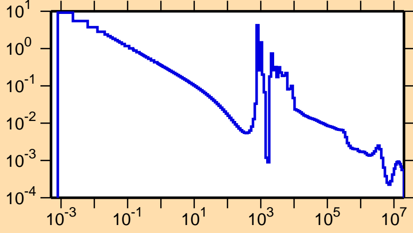
\sigma vs. E for ^{142}\text{Ba}(n,\gamma)
