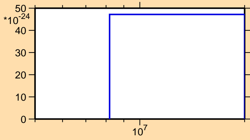
\sigma vs. E for ^{142}\text{Ba} (mt 11)
