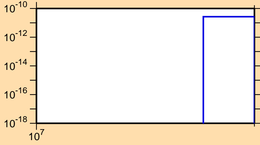
\sigma vs. E for ^{144}\text{Ba}(n,2np)
