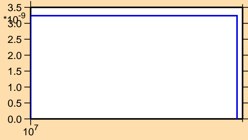
\sigma vs. E for ^{144}\text{Ba}(n,2n\alpha)
