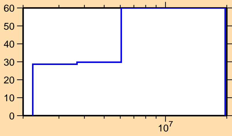
\Delta\sigma/\sigma vs. E for ^{144}\text{Ba}(n,\gamma)
