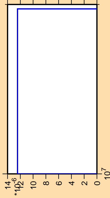
\Delta\sigma/\sigma vs. E for ^{144}\text{Ba} (mt 11)
