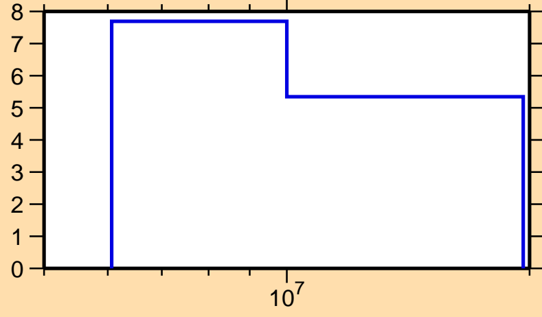
\Delta\sigma/\sigma vs. E for ^{144}\text{Ba}(n,\text{tot.})
