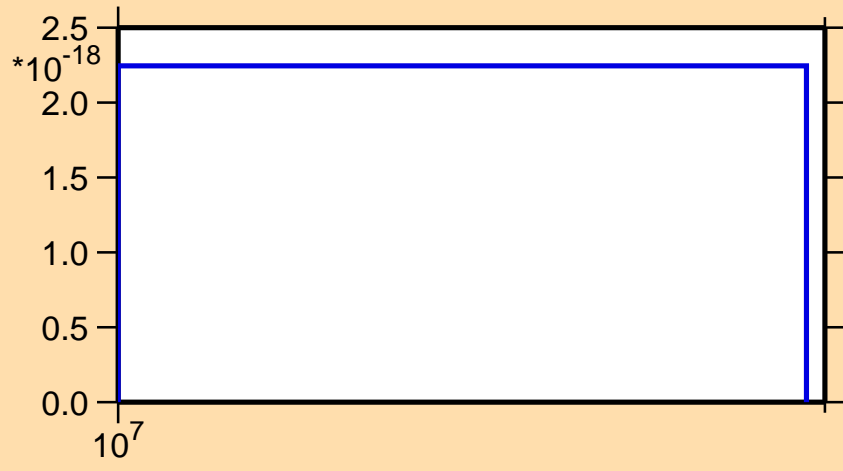
\sigma vs. E for ^{144}\text{Ba} (mt 11)
