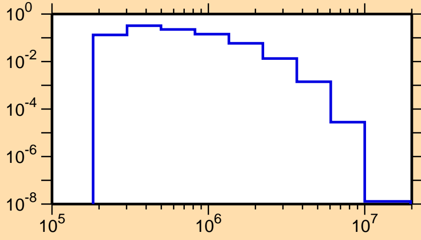
\sigma vs. E for ^{145}\text{Ba}(n,n_3)
