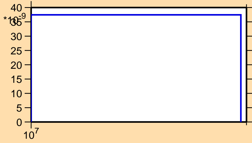
\sigma vs. E for ^{145}\text{Ba}(n,nt)
