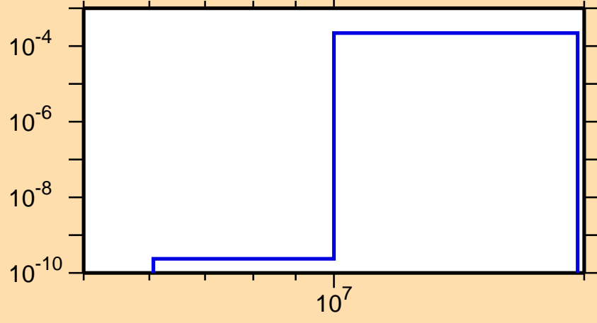
\sigma vs. E for ^{145}\text{Ba}(n,p)
