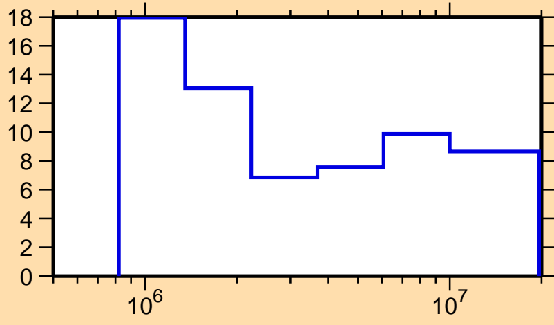
\Delta\sigma/\sigma vs. E for ^{145}\text{Ba}(n,n\text{onel.})
