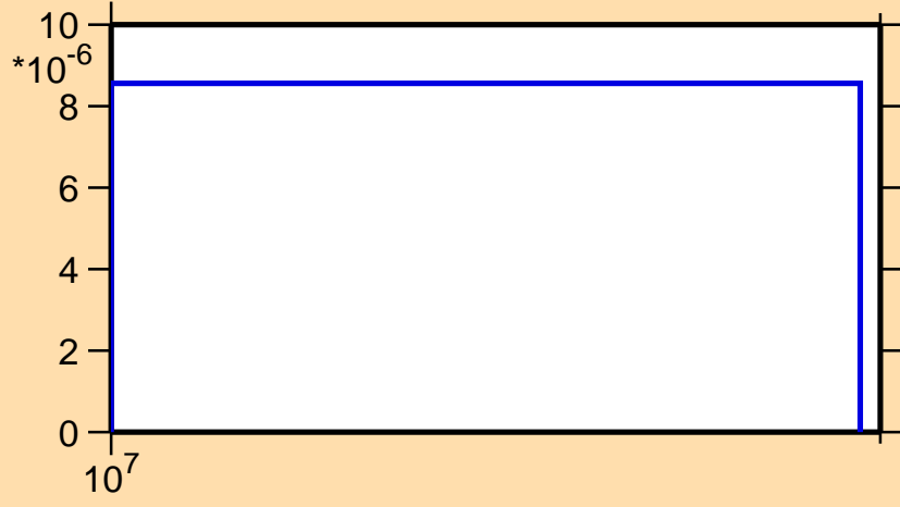
\sigma vs. E for ^{145}\text{Ba}(n,d)
