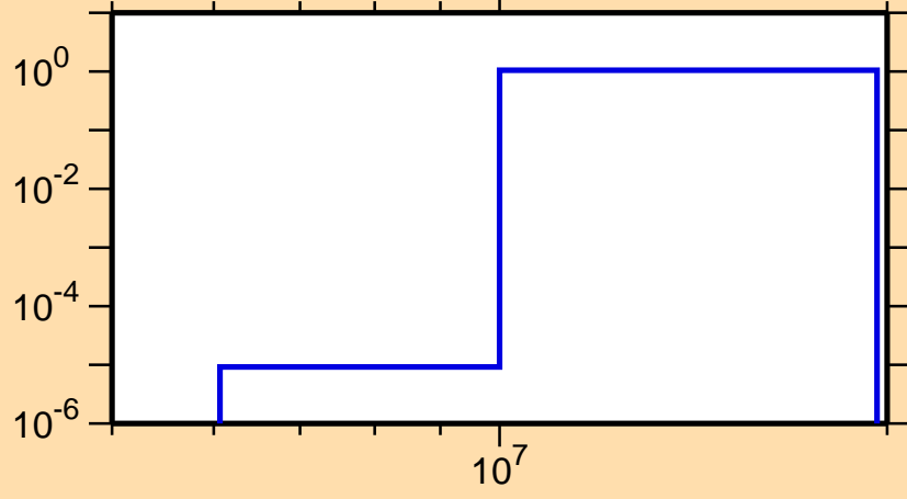
\sigma vs. E for ^{145}\text{Ba}(n,3n)
