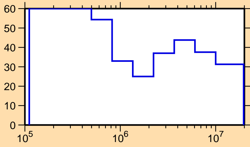
\Delta\sigma/\sigma vs. E for ^{145}\text{Ba}(n,n_1)
