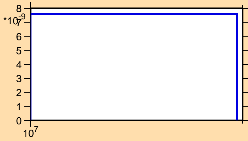
\sigma vs. E for ^{145}\text{Ba}(n,\text{nd})
