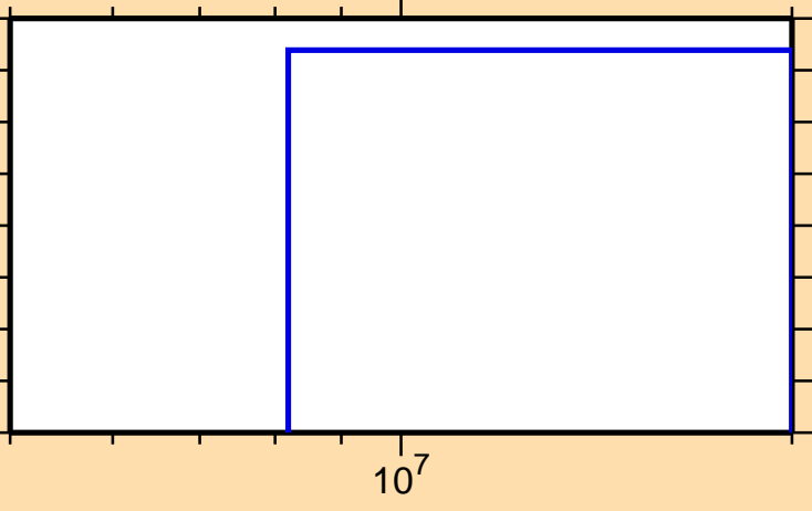
\sigma vs. E for ^{145}\text{Ba}(n,\text{nd})
