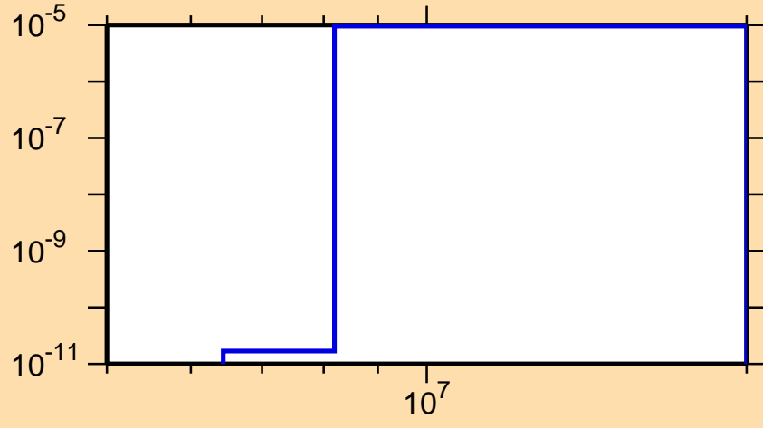
\sigma vs. E for ^{146}\text{Ba}(n,\alpha)
