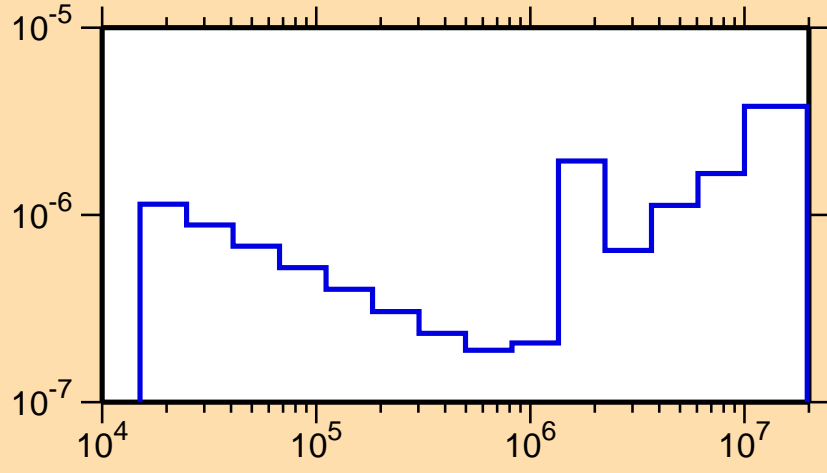
\sigma vs. E for ^{10}\text{Be}(n,\gamma)
