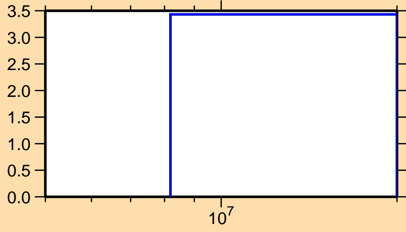
\Delta\sigma/\sigma vs. E for ^{10}\text{Be}(n,n\text{onel.})
