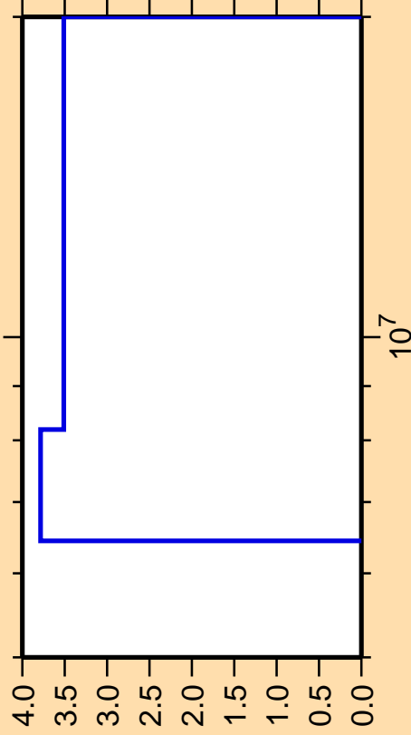
\Delta\sigma/\sigma vs. E for ^{10}\text{Be}(n,n_2)
