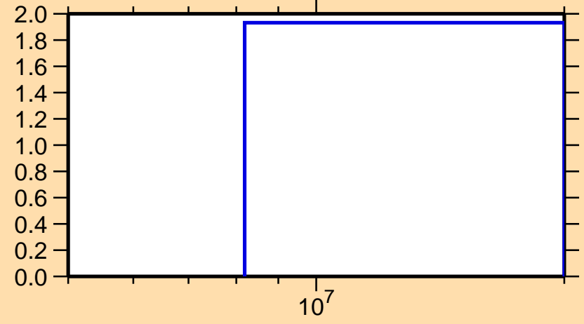
\Delta\sigma/\sigma vs. E for ^{11}\text{Be}(n,\text{el.})
