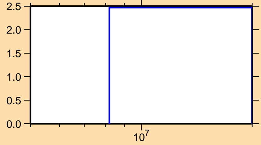
\Delta\sigma/\sigma vs. E for ^{11}\text{Be}(n,\text{inel.})
