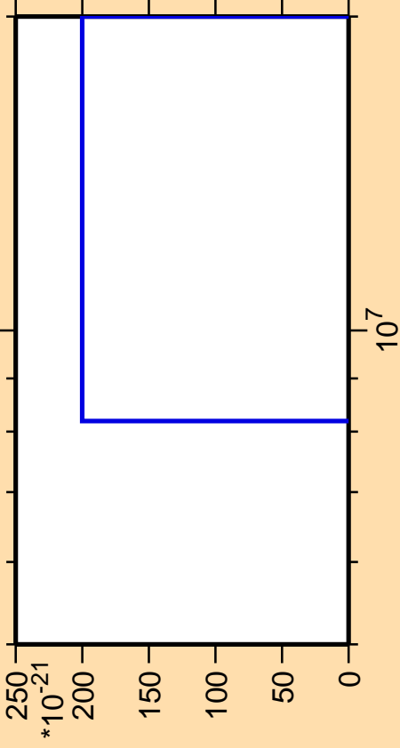
\Delta\sigma/\sigma vs. E for ^{11}\text{Be}(n,2n)
