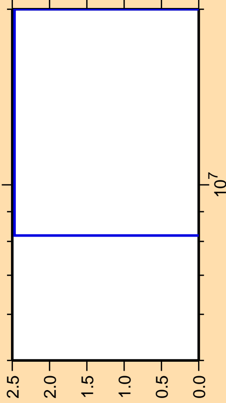
\Delta\sigma/\sigma vs. E for ^{11}\text{Be}(n,\text{inel.})
