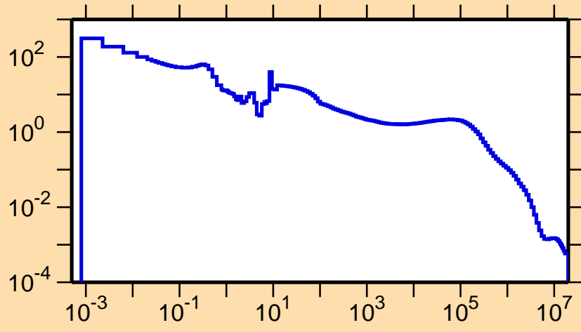
\sigma vs. E for ^{266}\gamma
