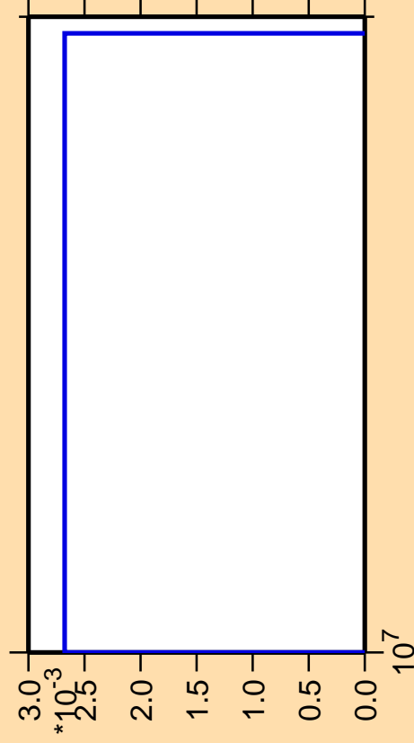
\Delta\sigma/\sigma vs. E for ^{274}\text{He3}
