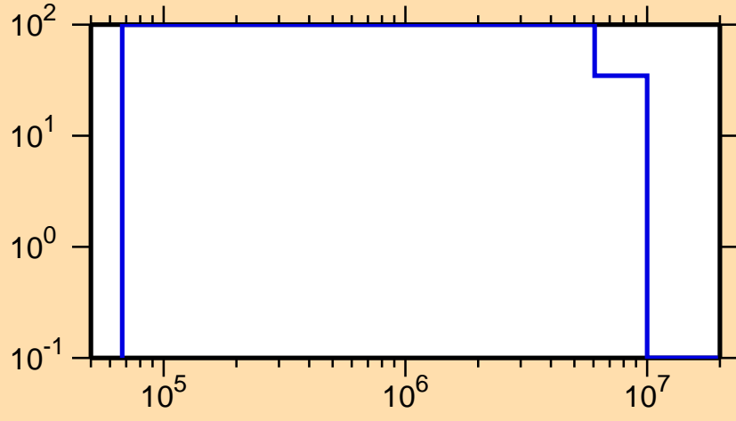
\Delta\sigma/\sigma vs. E for ^{274}_1
