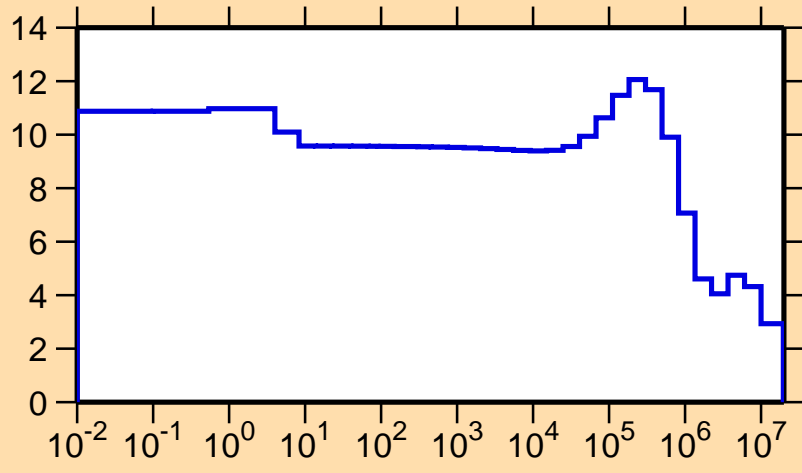
\sigma vs. E for ^{274}
