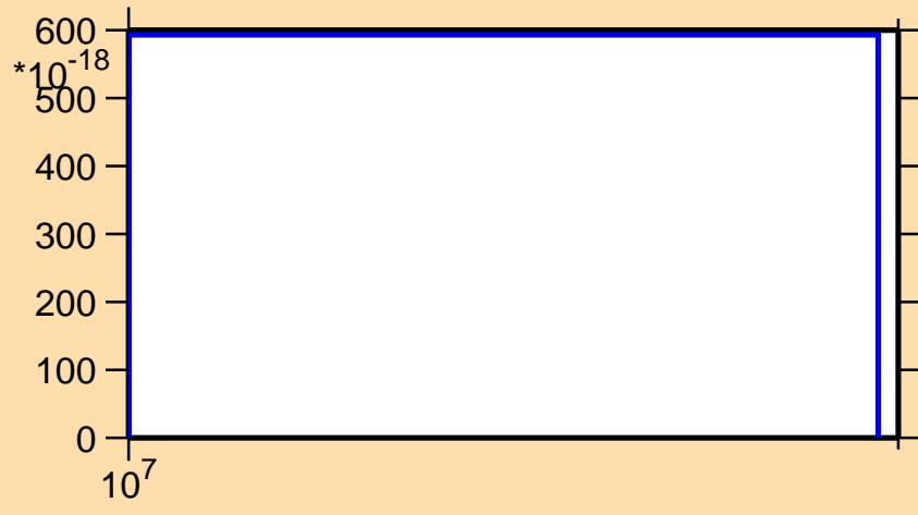
\sigma vs. E for ^{274}\text{He3}
