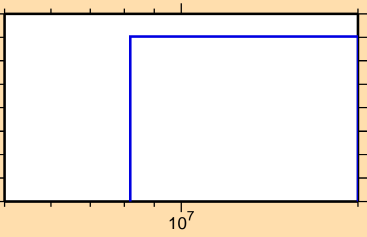
\sigma vs. E for ^{274}
