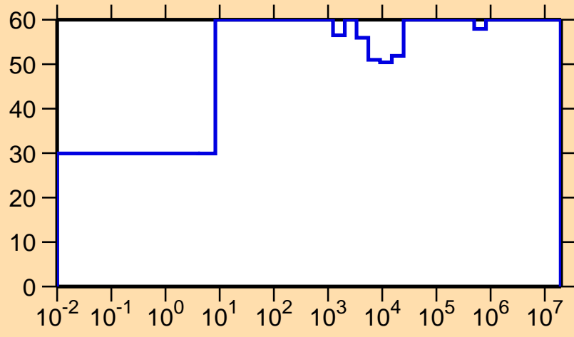
\Delta\sigma/\sigma vs. E for ^{275}\gamma
