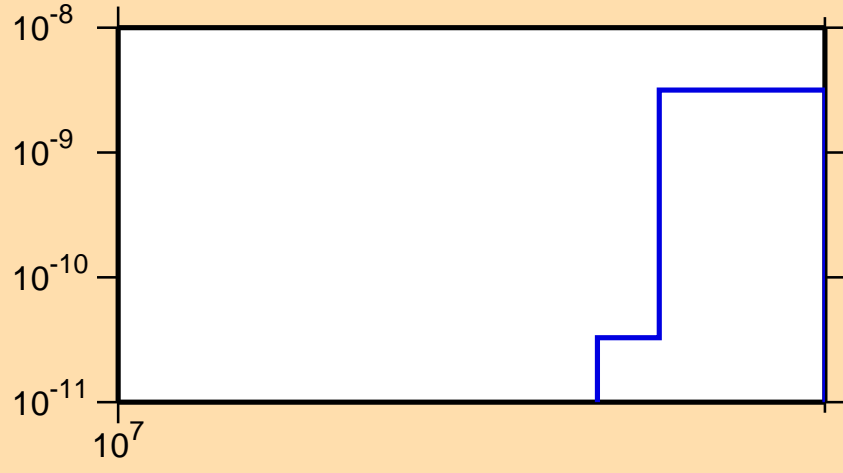
\sigma vs. E for ^{190}\text{Bi}(n,nt)
