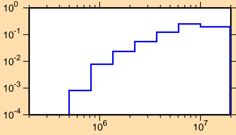
\sigma vs. E for ^{190}\text{Bi}(n,n\text{cont.})
