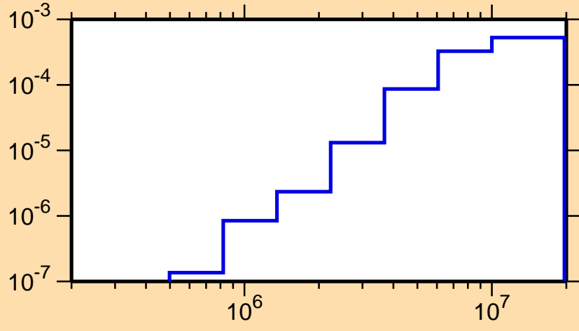
\sigma vs. E for ^{190}\text{Bi}(n,n_4)
