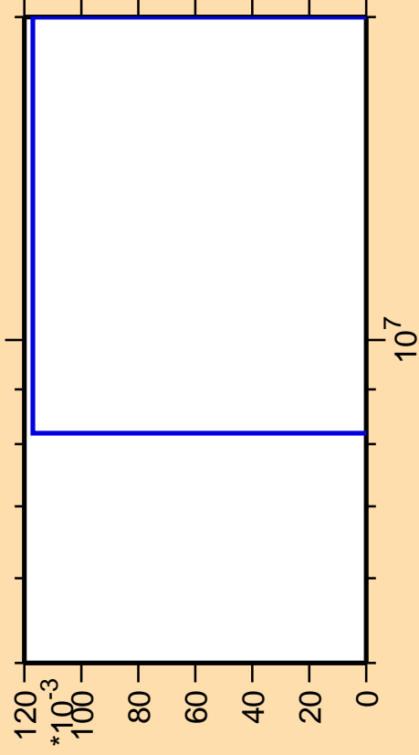
\Delta\sigma/\sigma vs. E for ^{190}\text{Bi}(n,3n)
