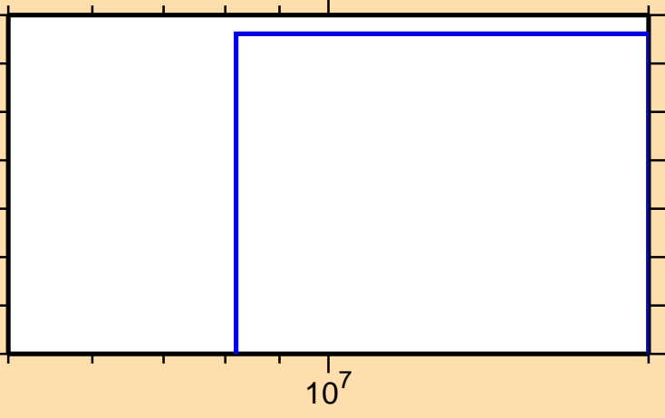
\sigma vs. E for ^{190}\text{Bi}(n,\text{pt})
