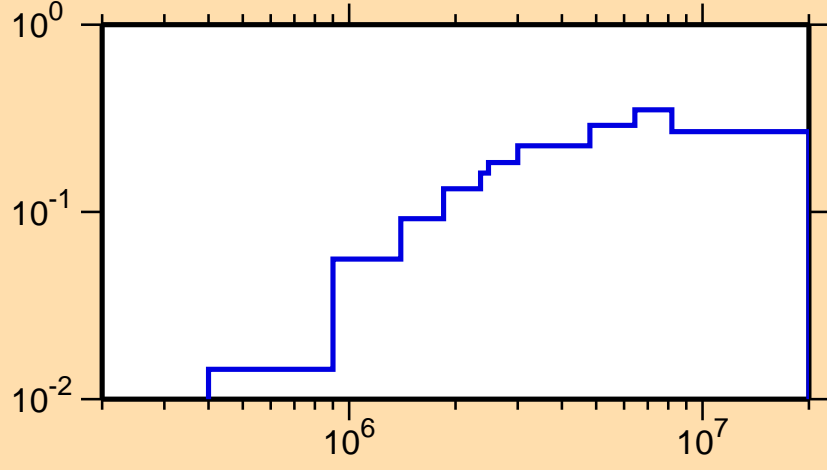
\sigma vs. E for ^{190}\text{Bi}(n,\text{inel.})
