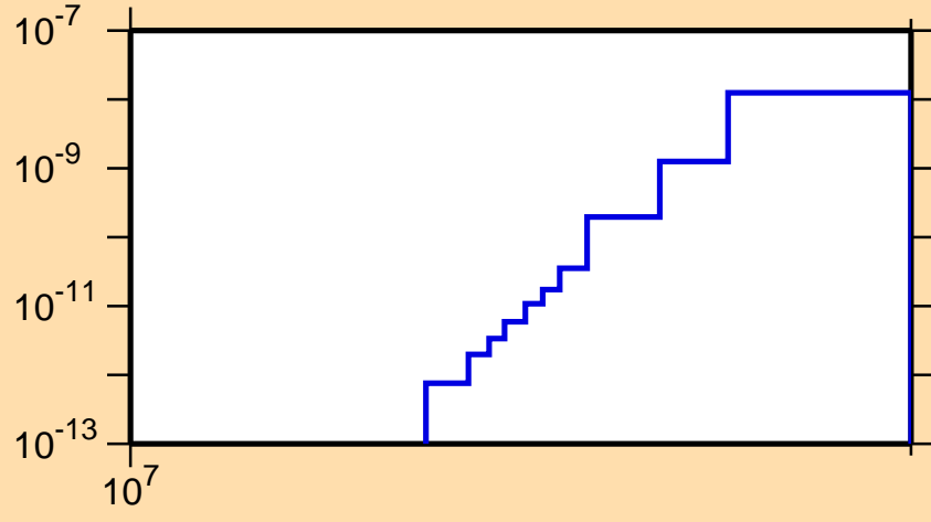
\sigma vs. E for ^{190}\text{Bi}(\text{mt } 34)
