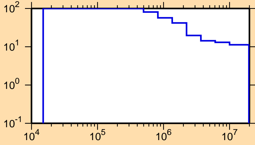
\Delta\sigma/\sigma vs. E for ^{190}\text{Bi}(n,n\text{nonel.})
