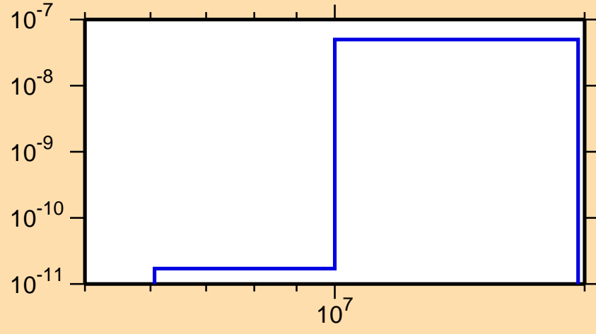
\sigma vs. E for ^{190}\text{Bi}(\text{mt117})
