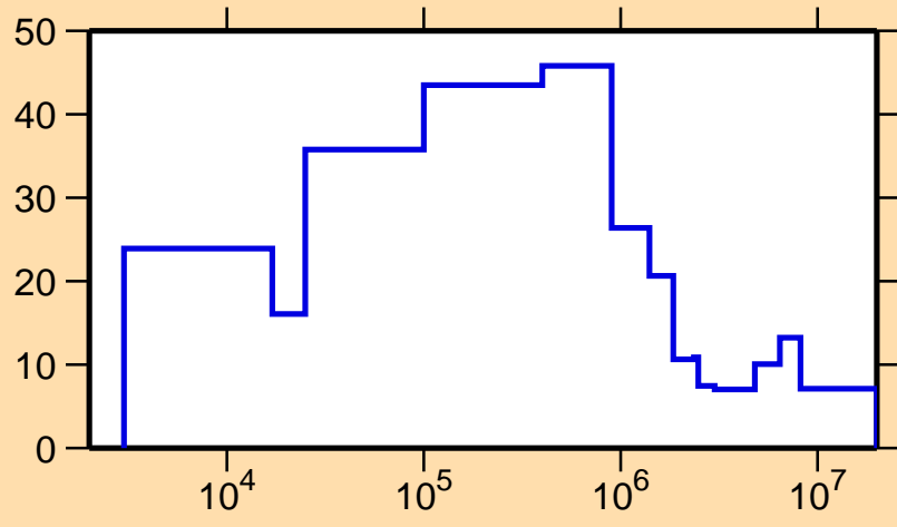
\Delta\sigma/\sigma vs. E for ^{190}\text{Bi}(n,\text{tot.})
