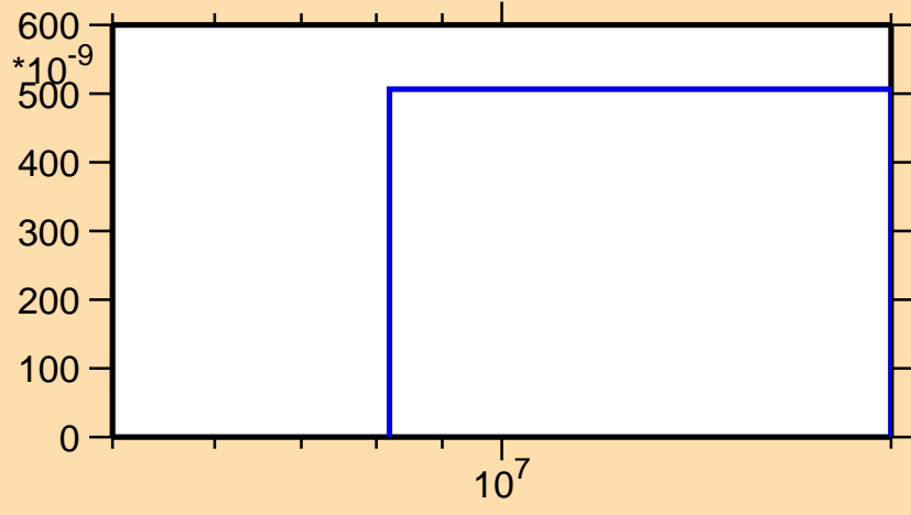
\sigma vs. E for ^{190}\text{Bi}(n,\text{nd})
