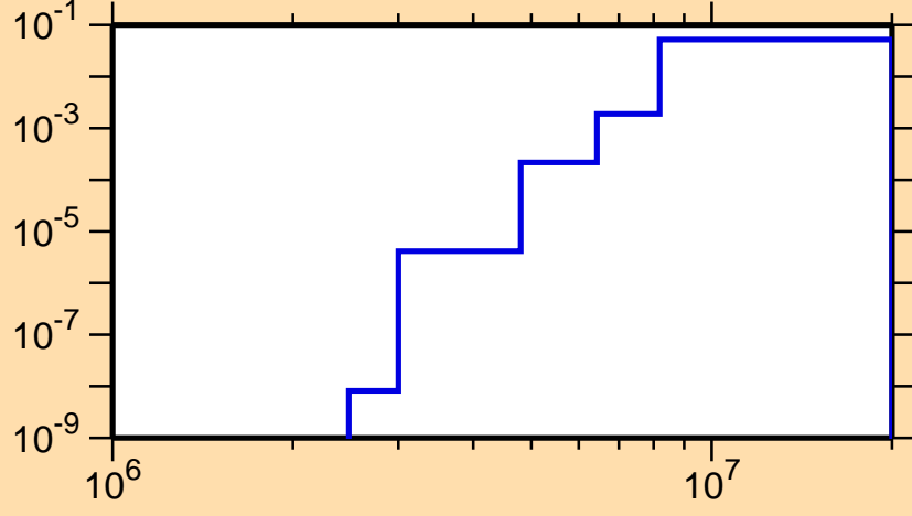
\sigma vs. E for ^{190}\text{Bi}(n,np)
