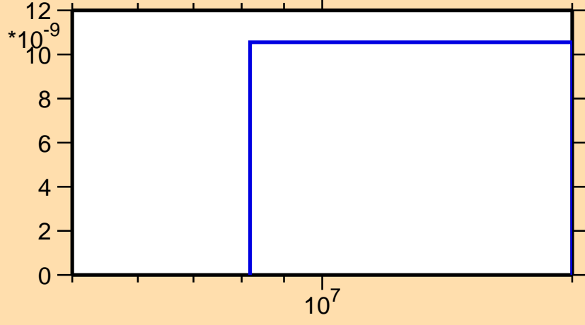
\sigma vs. E for ^{190}\text{Bi}(n,\text{pt})
