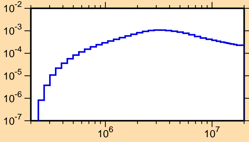
\sigma vs. E for ^{191}\text{Bi}(n,n_2)
