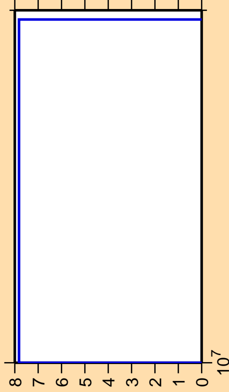
\Delta\sigma/\sigma vs. E for ^{192}\text{Bi}(n,3n\alpha)
