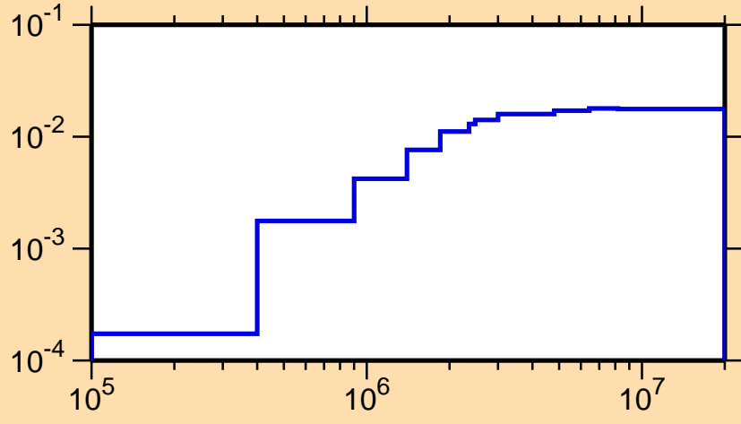
\sigma vs. E for ^{192}\text{Bi}(n,n_4)
