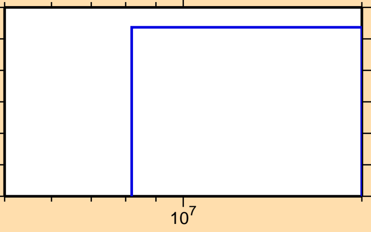
\sigma vs. E for ^{192}\text{Bi}(n,3n\alpha)
