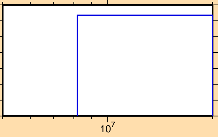
\sigma vs. E for ^{192}\text{Bi}(\text{mt117})
