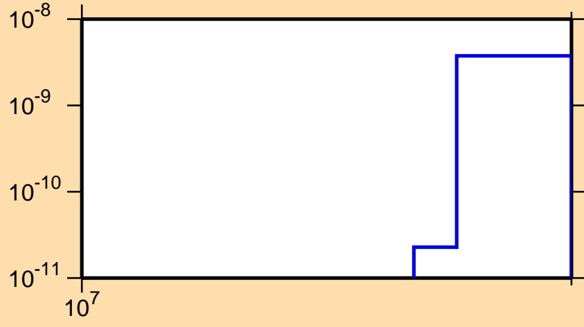
\sigma vs. E for ^{192}\text{Bi}(n,nt)
