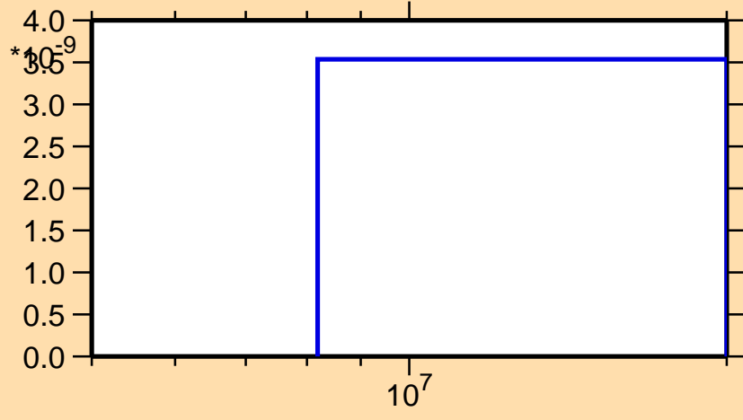
\sigma vs. E for ^{192}\text{Bi}(\text{mt117})
