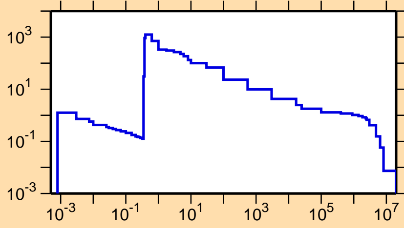
\sigma vs. E for ^{192}\text{Bi}(n,\gamma)
