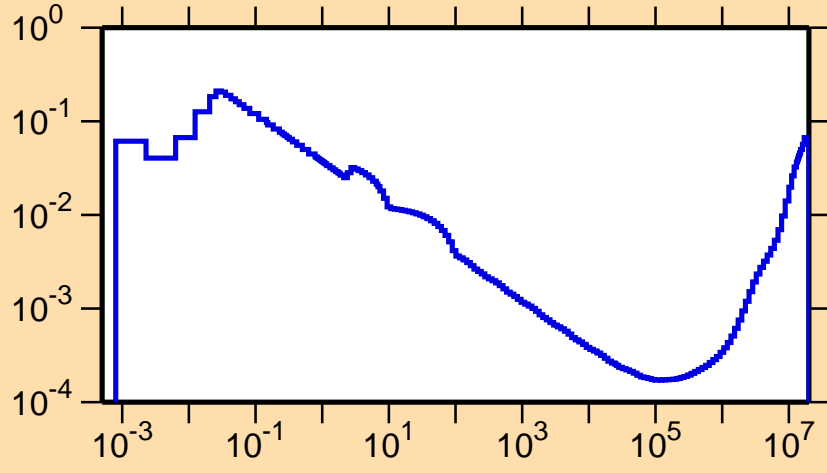
\sigma vs. E for ^{193}\text{Bi}(n,\alpha)
