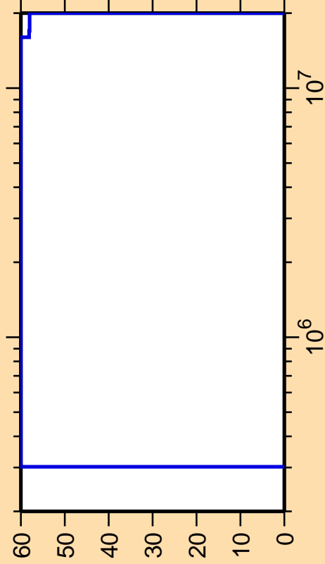
\Delta\sigma/\sigma vs. E for ^{193}\text{Bi}(n,n_1)
