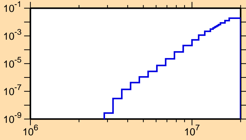
\sigma vs. E for ^{193}\text{Bi}(n,n\alpha)
