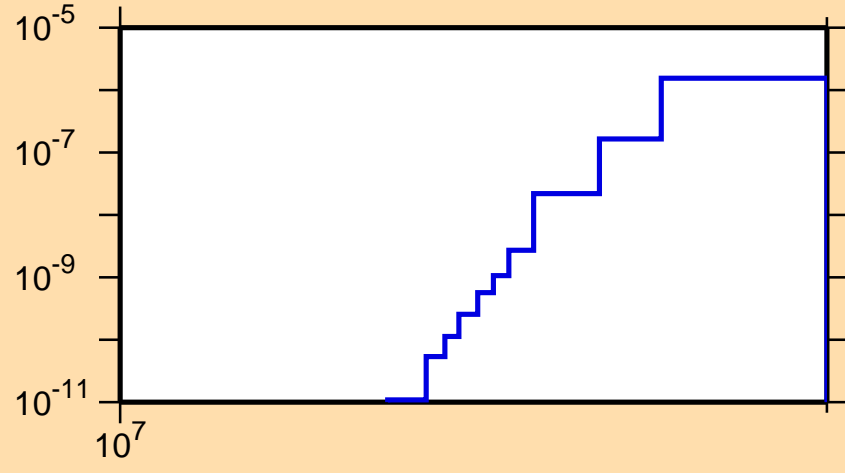
\sigma vs. E for ^{193}\text{Bi}(n,\text{nd})
