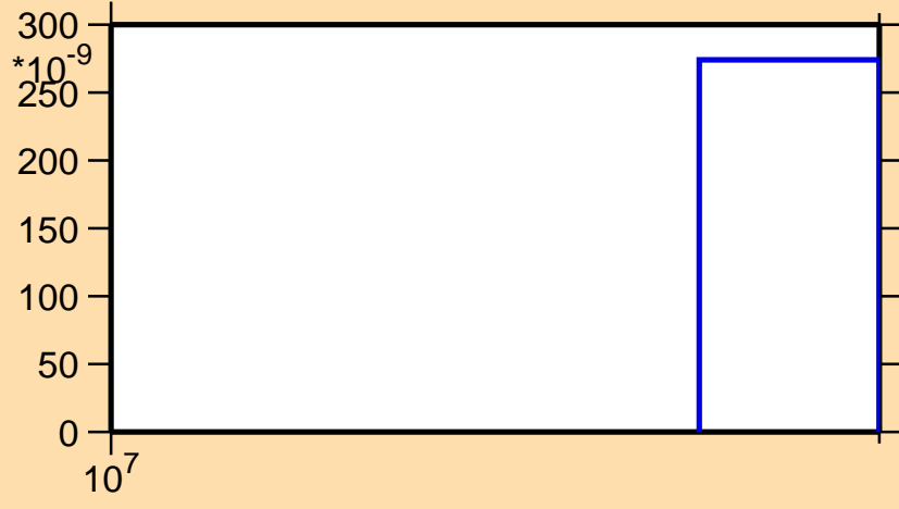
\sigma vs. E for ^{193}\text{Bi}(n,3n)
