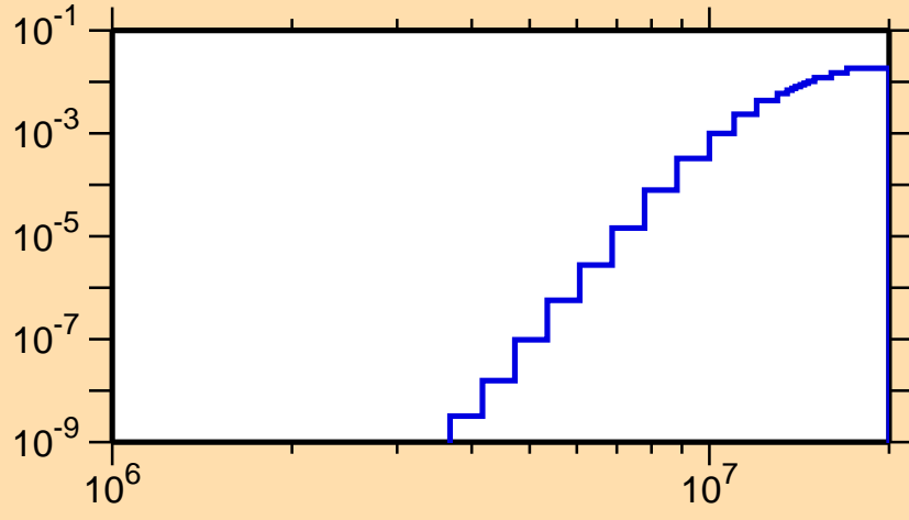
\sigma vs. E for ^{193}\text{Bi}(n,d)
