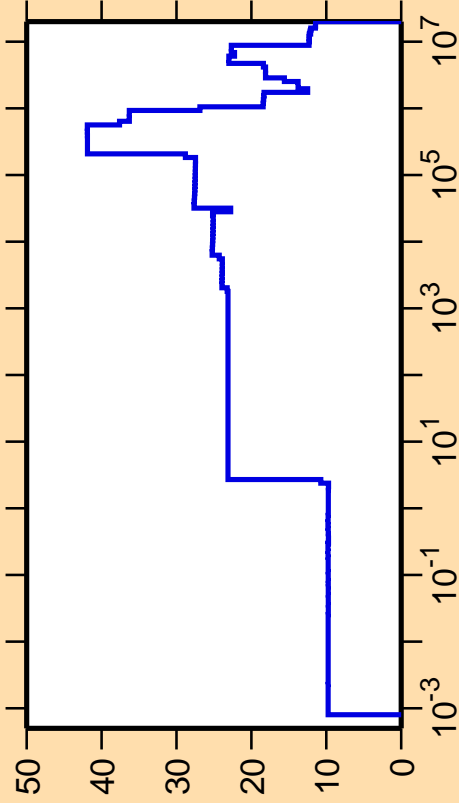
\Delta\sigma/\sigma vs. E for ^{193}\text{Bi}(n,\text{el.})
