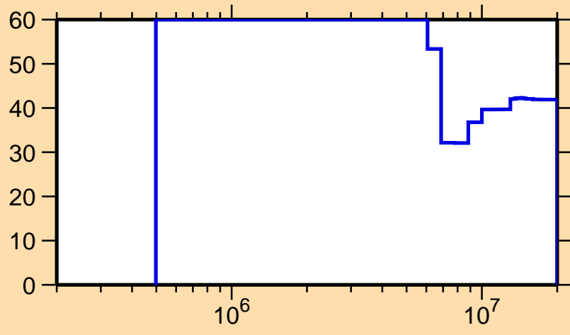
\Delta\sigma/\sigma vs. E for ^{193}\text{Bi}(n,n\text{cont.})
