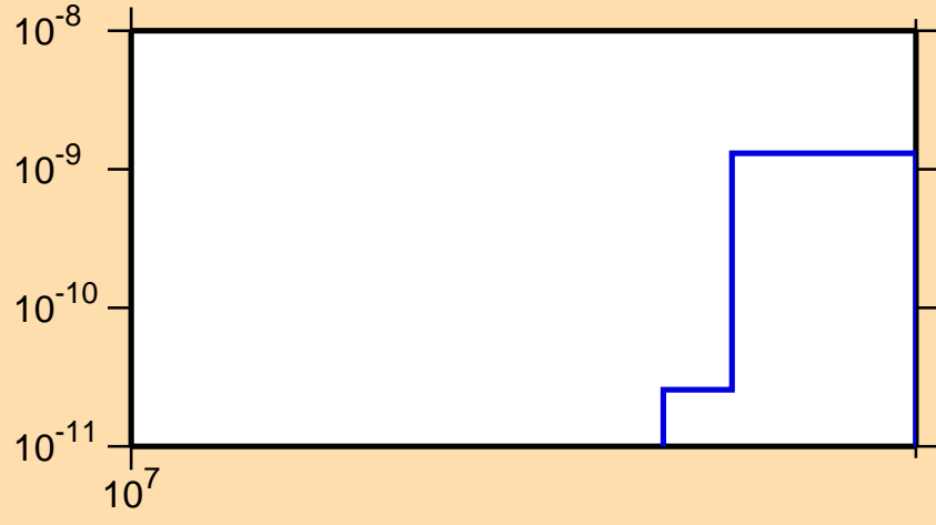
\sigma vs. E for ^{193}\text{Bi}(n,\text{pt})
