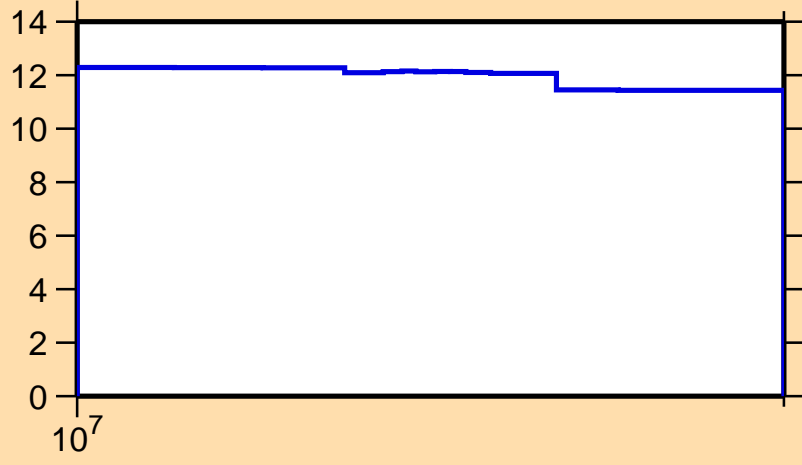
\Delta\sigma/\sigma vs. E for ^{193}\text{Bi}(n,\text{el.})
