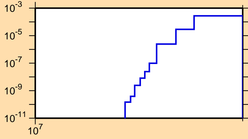
\sigma vs. E for ^{193}\text{Bi}(n,2np)
