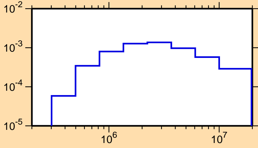
\sigma vs. E for ^{193}\text{Bi}(n,n_1)
