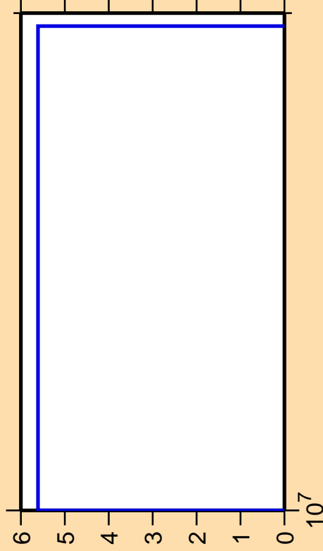
\Delta\sigma/\sigma vs. E for ^{193}\text{Bi} (mt 34)
