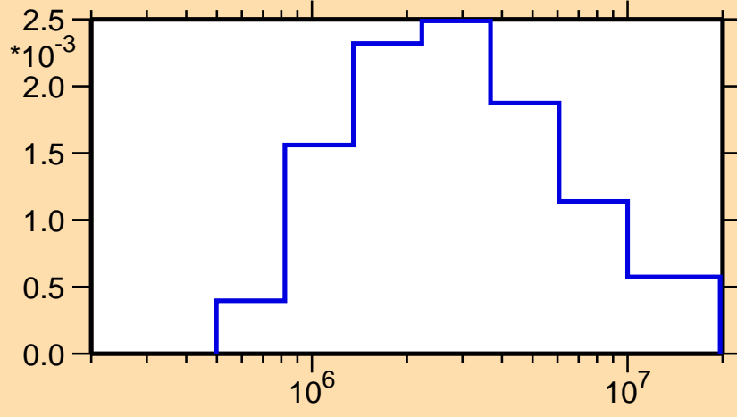
\sigma vs. E for ^{193}\text{Bi}(n,n_2)
