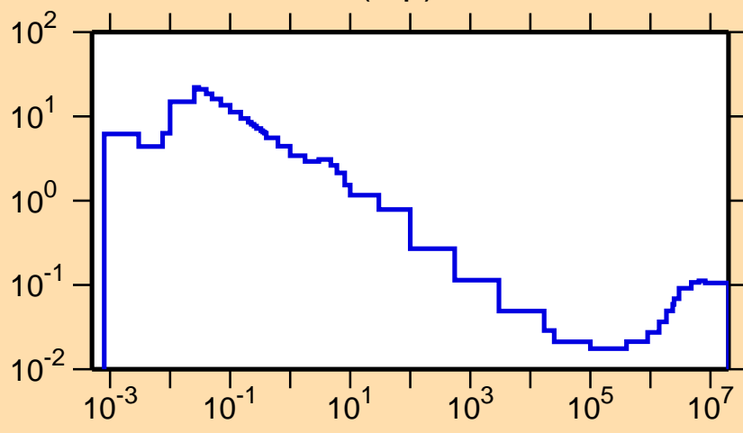
\sigma vs. E for ^{193}\text{Bi}(n,p)
