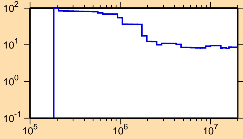
\Delta\sigma/\sigma vs. E for ^{193}\text{Bi}(n,n\text{nonel.})
